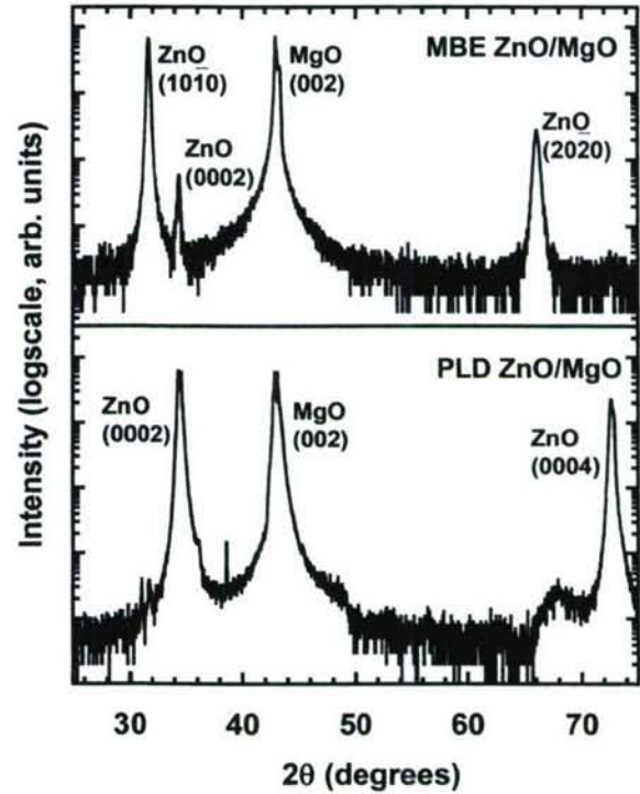
Figure 8: X-ray diffraction \theta -2 \theta scan demonstrating m-plane orientation for MBE growth of ZnO on MgO and c-plane growth for deposition by laser ablation (layer thickness approximately 0.1 \mu\text{m} each layer).
