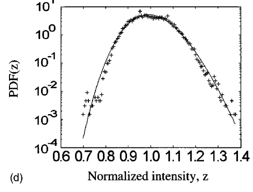
Fig. 5 Experimentally determined PDF( z ) versus z for a retroreflector spacing of 20 mm with lens aperture diameter as a parameter. Solid curves represent lognormal PDF. Parameter values are (a) D_R=3 mm, \sigma_{\ln z}^2=1.09 \times 10^{-1} , \Delta z=2.39 \times 10^{-2} ; (b) D_R=10 mm, \sigma_{\ln z}^2=5.38 \times 10^{-3} , \Delta z=5.96 \times 10^{-3} ; (c) D_R=20 mm, \sigma_{\ln z}^2=6.61 \times 10^{-3} , \Delta z=6.06 \times 10^{-3} ; (d) D_R=30 mm, \sigma_{\ln z}^2=6.02 \times 10^{-3} , \Delta z=5.89 \times 10^{-3} .
