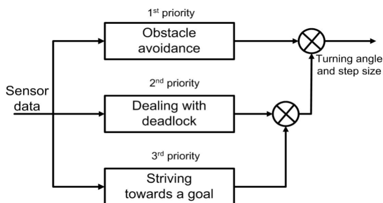
Figure 1: Subsumption architecture
