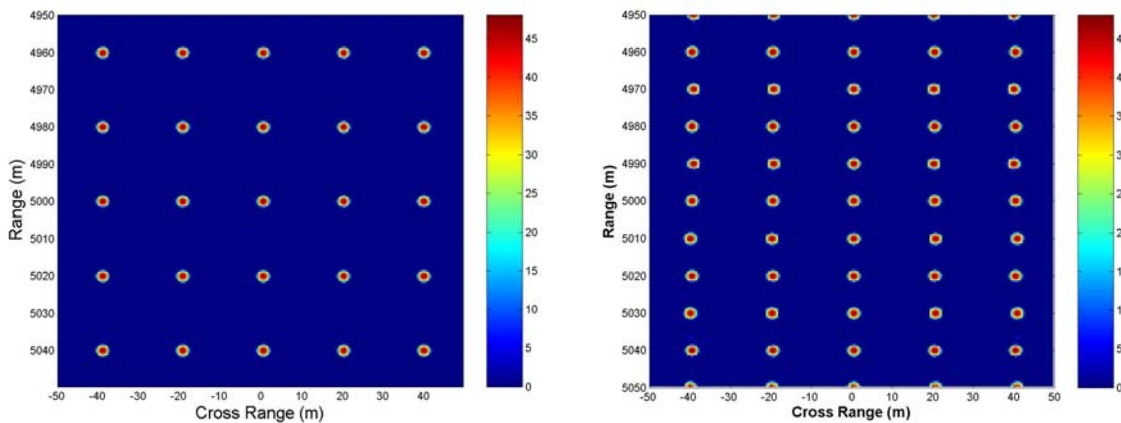
Figure 1: (Left) Range-unambiguous SAR image of a grid of 25 point scatterers over an 80m x 80m area using a full frequency set. The intensity range is 48dB. (Right) Using a simple linear re-sampling of the 101 frequencies used in Figure 1 to 51 frequencies, with an increased \Delta f=3.0\text{MHz} to cover the bandwidth. The reduction of the unambiguous range to 50m has produced strong range-ambiguities.
