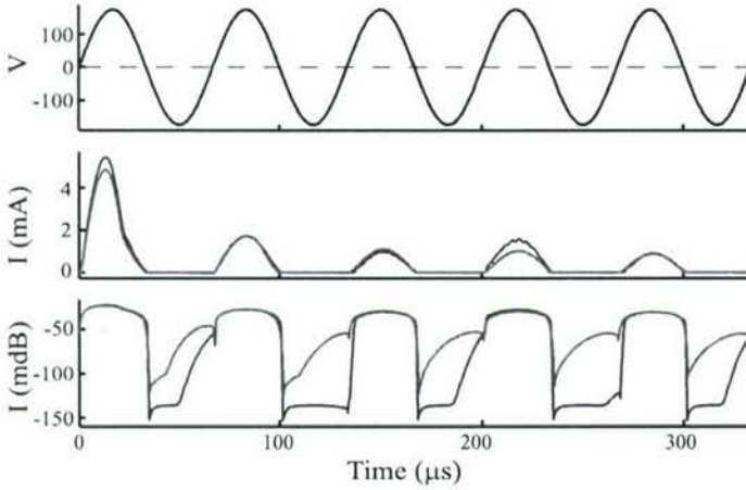
Figure 17: Current-voltage relationship for isotropic plasma with sinusoidal applied potential at 15kHz. 'Blue' - 2 moments. 'Red' - 3 moments.
