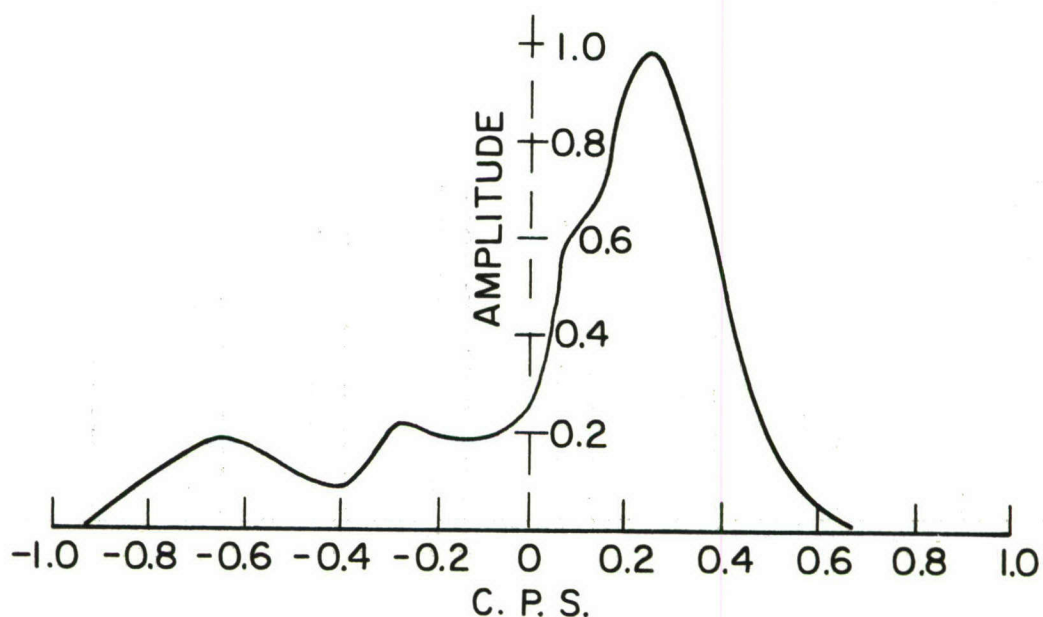
Figure A3 - Fourier-type analysis with one-tenth cycle bandwidth filter taken of a 20-second sample of backscatter. Frequency with 18 Mc, bearing 082°T, 10° beamwidth and sample 20-mile length range gated at 1400 naut. mi.
