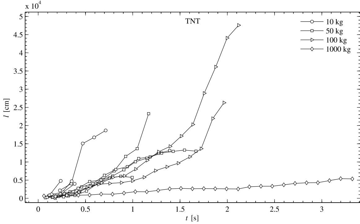
Figure 46: Photon mean free path l versus time for the TNT fireballs, grouped according to weight: 10 ( \circ ), 50 ( \square ), 100 ( \triangleright ), and 1000 kg ( \diamond ).
