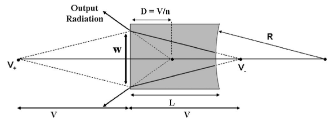
FIG. 2. Schematic of unstable resonator showing virtual source points V_+ and V_- . L is the resonator length (3.5 mm), R is the radius of curvature of the polished cylinder \approx 10 mm, w is the stripe width (full width at half maximum = 250 \mu\text{m} ) and D is the refractively reduced distance to the virtual source, D = 1810 \mu\text{m} .
