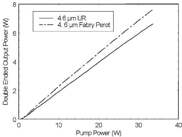
FIG. 1. Peak power-power curves for L=3.5 mm long Fabry-Pérot and unstable resonator lasers operating near 4.6 \mu\text{m} and 84 K. To minimize thermal load on the laser the curves were collected under pulsed conditions: 32 \mu\text{s} pulse, 1% duty cycle.
