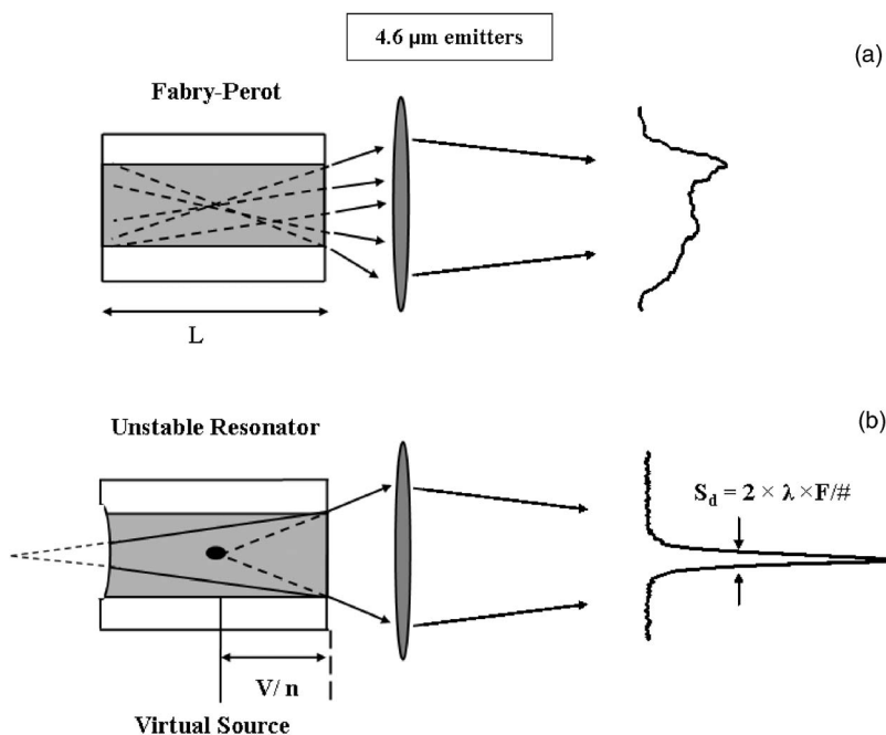
FIG. 3. (a). Reimage of degraded best focus at 30 times threshold for the Fabry-Pérot laser. (b) Reimage of virtual source at 25 times threshold for the 4.6 \mu\text{m} UR. The virtual source size indicates that the lateral mode is nearly diffraction limited.
