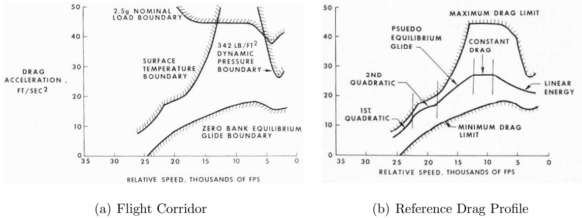
Figure 1: Shuttle Entry - Operational Angle-of-Attack Profile. [39]
