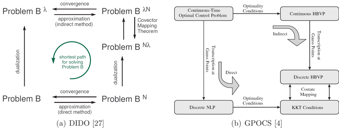
Figure E.5: Computation of the Continuous Lagrange Multipliers
