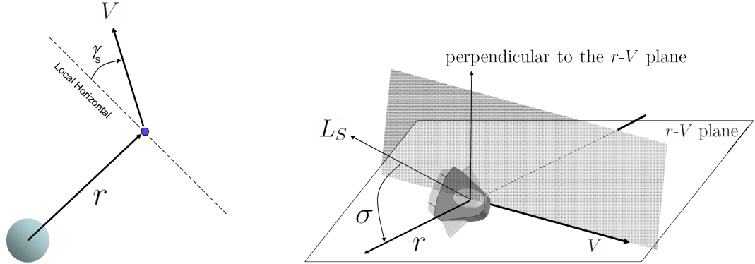
Figure B.1: Fight Path Angle [41] Figure B.2: Schematic of the r - V plane [41]
