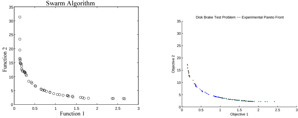
(a) Pareto Front for Deterministic Test Problem, Figure 6 in [119]
