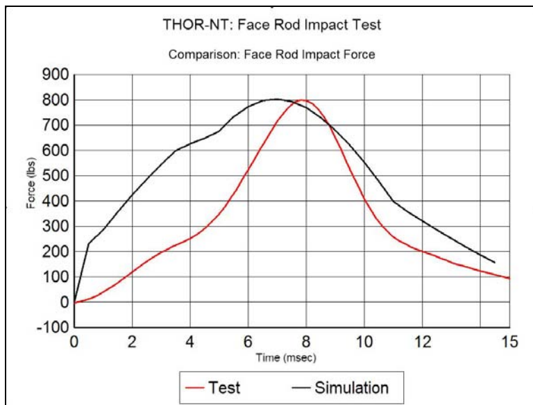
Figure 10: Comparison of Test and Simulation Force for Face Rod Impact
