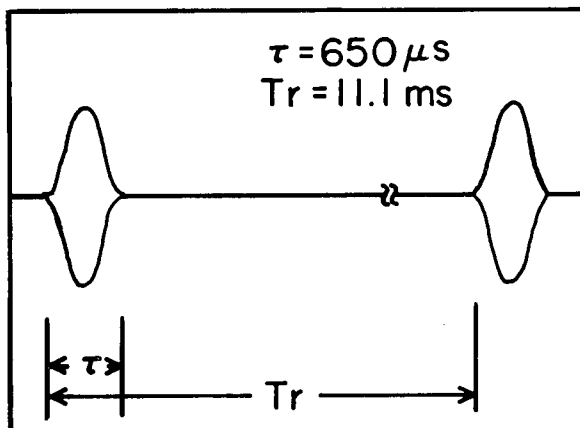
Fig. 6 - Transmitter output waveform
