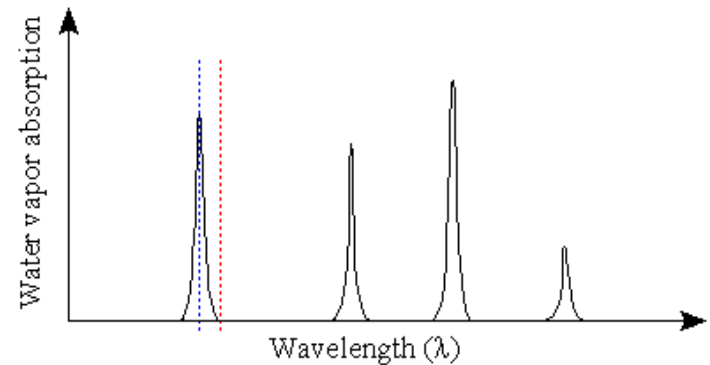
(a) Water vapor absorption spectrum
