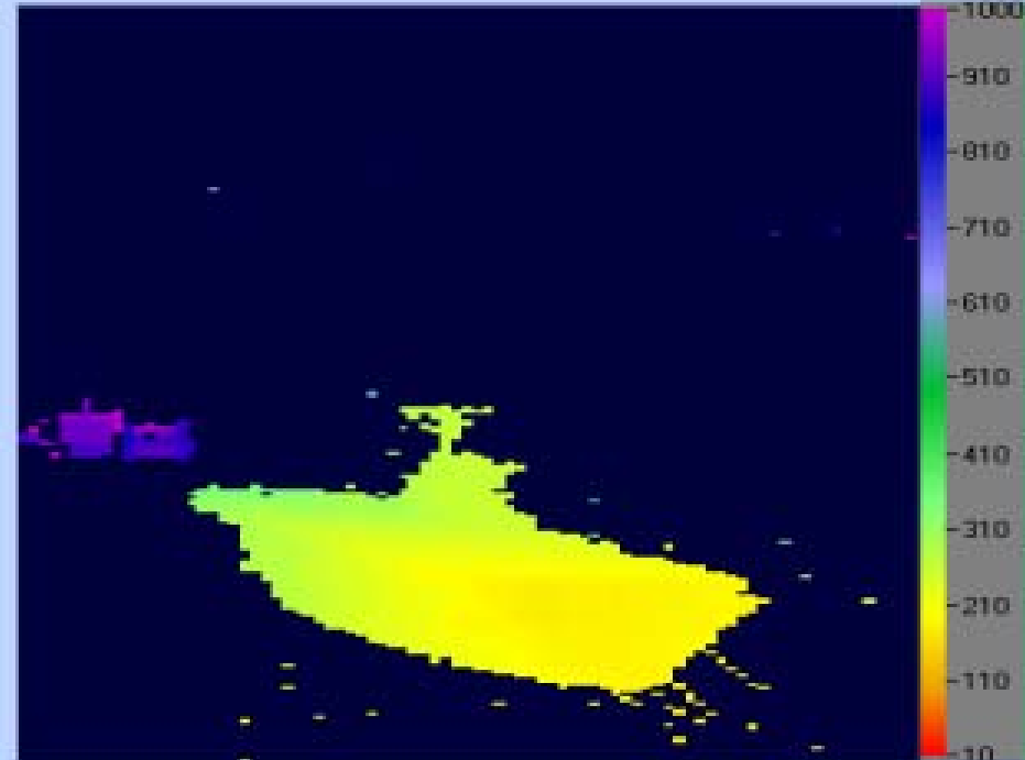
Hellas LADAR
