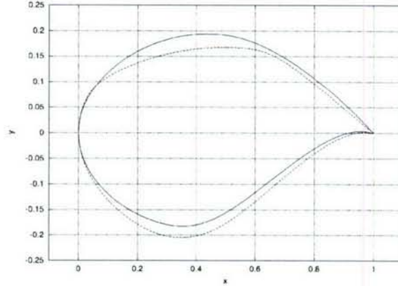
Figure 19: RAE-82 optimized for minimum drag at Mach 0.77: Original (solid) and Optimized (dotted)
