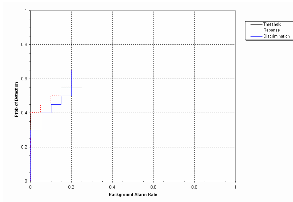
Figure 9. EM Sensor open field probability of detection for response and discrimination stages versus their respective background alarm rate for all ordnance larger than 20 mm.
