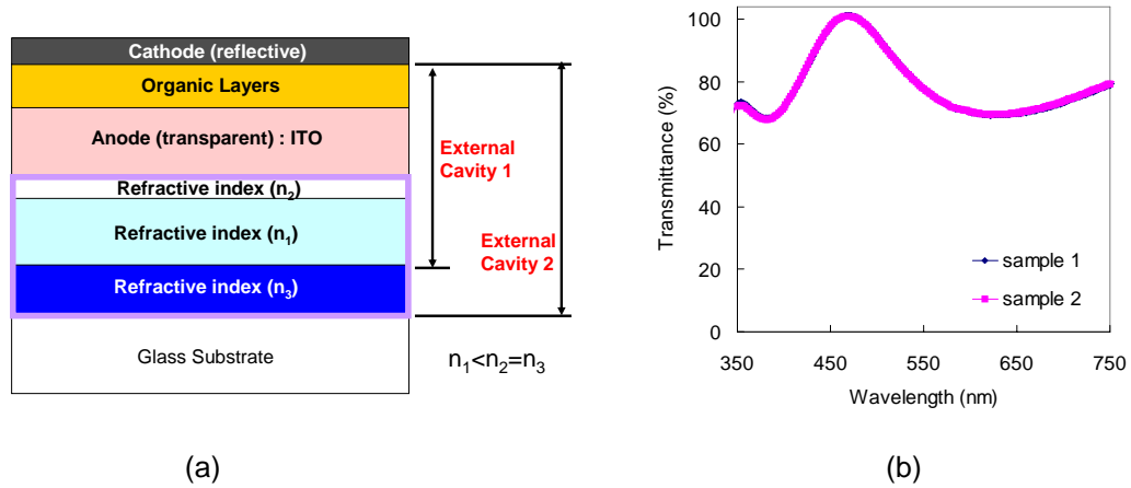
Figure 11 (a) Design of non-periodic microcavity structure (b) transmittance of dielectric mirror with structure of TiO 2 54nm /SiO 2 90nm /TiO 2 54nm /Glass
