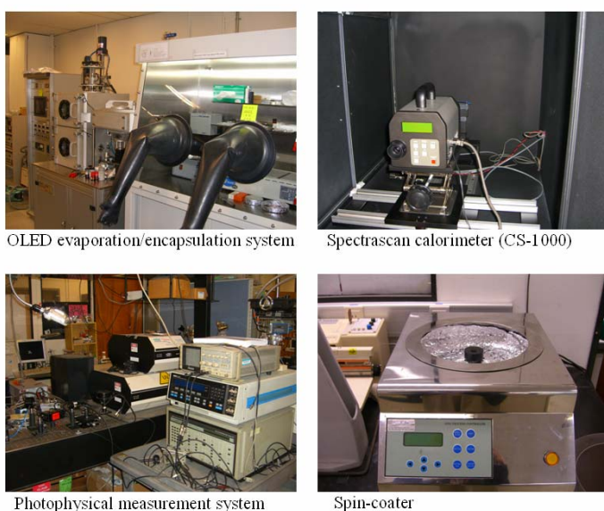
Figure 5. Experimental apparatus for OLED device fabrication and characterization
