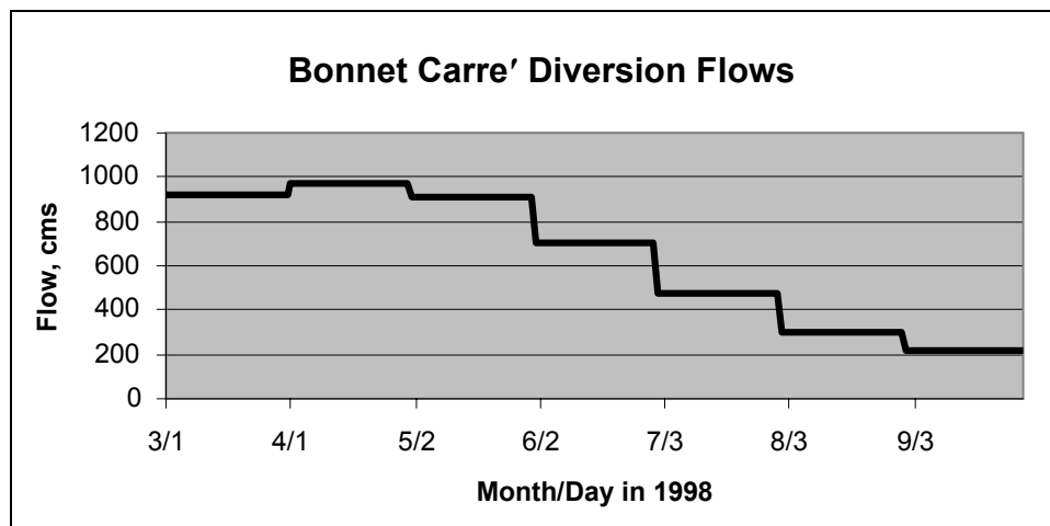
Figure 5-1. Bonnet Carré diversion flows.
