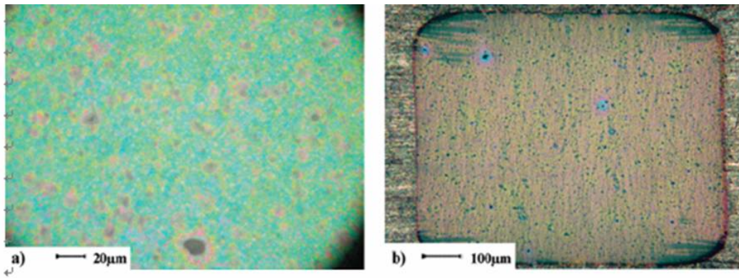
Figure 6. Optical micrograph of MWNT/PS films coated on copper grids: (a) local deformation zones initiated at 1.2% strain (the black spot at the bottom is a nanotube aggregate) and (b) many tiny local deformation zones at 23.5% strain.
