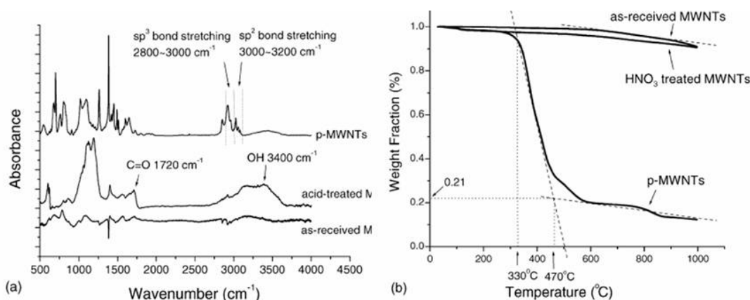
Figure 2. (a) The FTIR spectra of the as-received MWNTs, acid-treated MWNTs and graft polymerized MWNTs (p-MWNTs); (b) Thermogravimetric curves of the as-received MWNTs (purity > 96%), acid-treated MWNTs with nitric acid and p-MWNTs.
