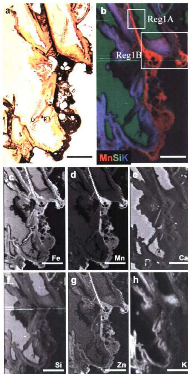
Figure 5.1. Characterization of EPR7A. (a) Light microscope image of the thin-section ( \sim 30\ \mu\text{m} thick) showing the transition from fresh glass (beige color) through the alteration layer (yellow-orange rind) and into the Fe- and Mn-oxide coated surface (black). (b) \mu\text{SXRF} tricolor map with Mn coded as red, Si as green, and K as blue. The white boxes outline the regions (1A and 1B) used for more detailed analyses. (c-f) Grayscale maps for elements Fe, Mn, Ca, Si, Zn, and K where bright colors indicate high concentrations. Scale bar is 500\ \mu\text{m} in all images.
