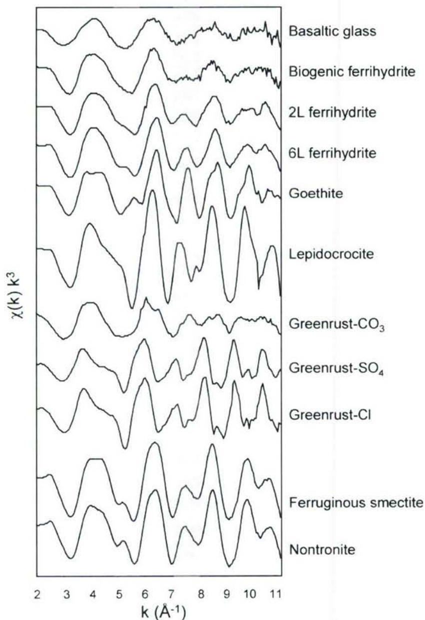
Figure 5.8. Summary of k^3 -weighted Fe EXAFS spectra of reference materials used for principal component analysis (PCA) and linear least-squares fitting. The gray boxes (indicator regions) highlight features relevant for distinguishing the Fe oxides and oxyhydroxides. The phase shifts and amplitude differences represent structural changes of these minerals.
