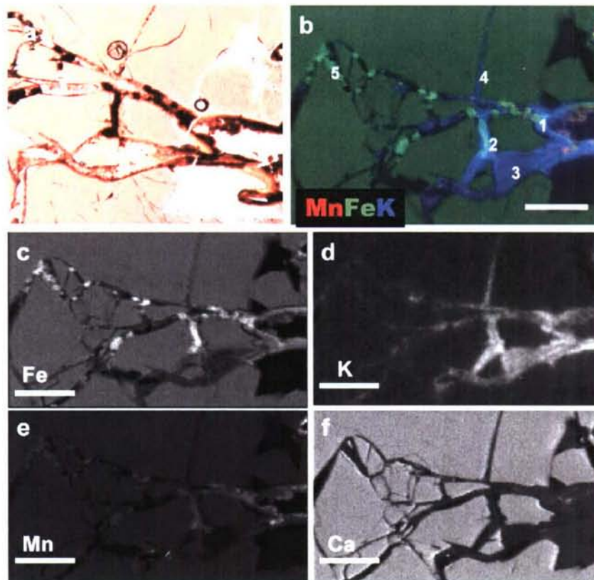
Figure 5.5. Elemental maps of EPR3970_Region3 (fractured glass filled with alteration products). (a) Light microscope image of the veins in thin-section. (b) \mu SXRF tricolor map with Mn coded as red, Fe as green, and K as blue. The numbers (1 -5) represent the locations of spot analyses used for Fe EXAFS measurements. (c-j) Grayscale maps for elements Fe, K, Mn, and Ca where bright colors indicate high concentrations. Scale bar is 400 \mu m in all images.
