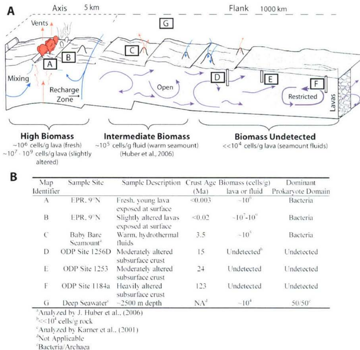
Figure 6.1. (A) Cross-sectional diagram of the upper portion (basaltic lava flows) of the ocean crust demonstrating the high prokaryotic biomass in young crust that generally decreases with increasing age of the crust (modified after Edwards et al., (2005)). Very young crust ( < 20 kyrs), however, shows an increase in biomass during initial stages of basalt alteration. Microbial communities in old, subsurface crust could not be detected using standard, molecular biological tools. Letter indicators on map are described in table below. (B) Table describing map identifier (letters A-G). All analyses are from this study unless indicated.
