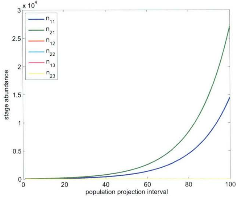
Figure 7-4: Without the epidemic, the structured population grows exponentially. Parameter values: g_i = 0.3 , m_1 = 0.2 , m_2 = 0.1 , f_i = 0.3 , initial conditions: \mathbf{n}_{\text{epidemic}} = (100 \ 50 \ 0 \ 0 \ 0 \ 0)^\top .
