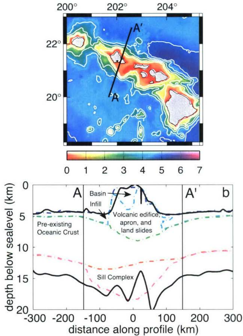
Figure 2-10: Crustal cross section across the island of Oahu. (a) Shiptrack bathymetry contoured every 1000 m with the A-A' profile used by ten Brink and Brocher [1987]. (b) Digitized interfaces from the crustal structure of the island of Oahu inferred from reflection and refraction marine seismic profiles collected around the island [Ten Brink and Brocher, 1987] (dash-dot lines) are compared with the shiptrack bathymetry and our gravity-derived crust-mantle interface (solid lines). Our calculated Moho (lower solid line) compares well with the seismic crustal thickness (lowest dash-dot line) near the seamount. At distances greater than 200 km from Oahu, the gravitational signal of the Hawaiian swell leads us to overpredict crustal thickness relative to the seismic interpretation. However, it is worth noting that the seismic interpretation is based on data that is confined between A and A' and is therefore not well constrained under the swell.
