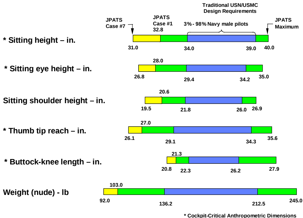
Figure 1: Past and Present USN Aircraft Accommodation Specification Criteria
