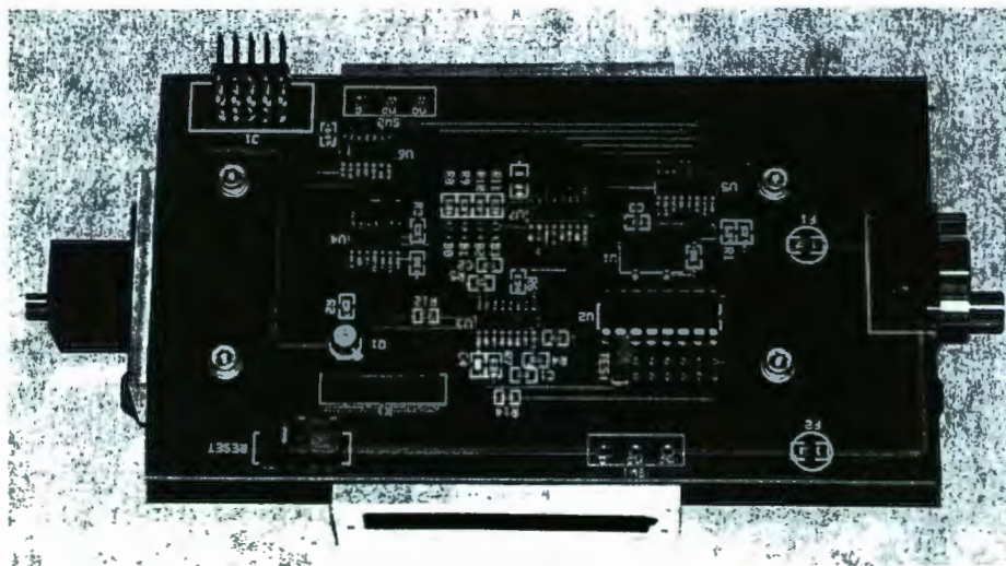
Figure 15. Electronics circuit for Notre Dame translator assembly.
