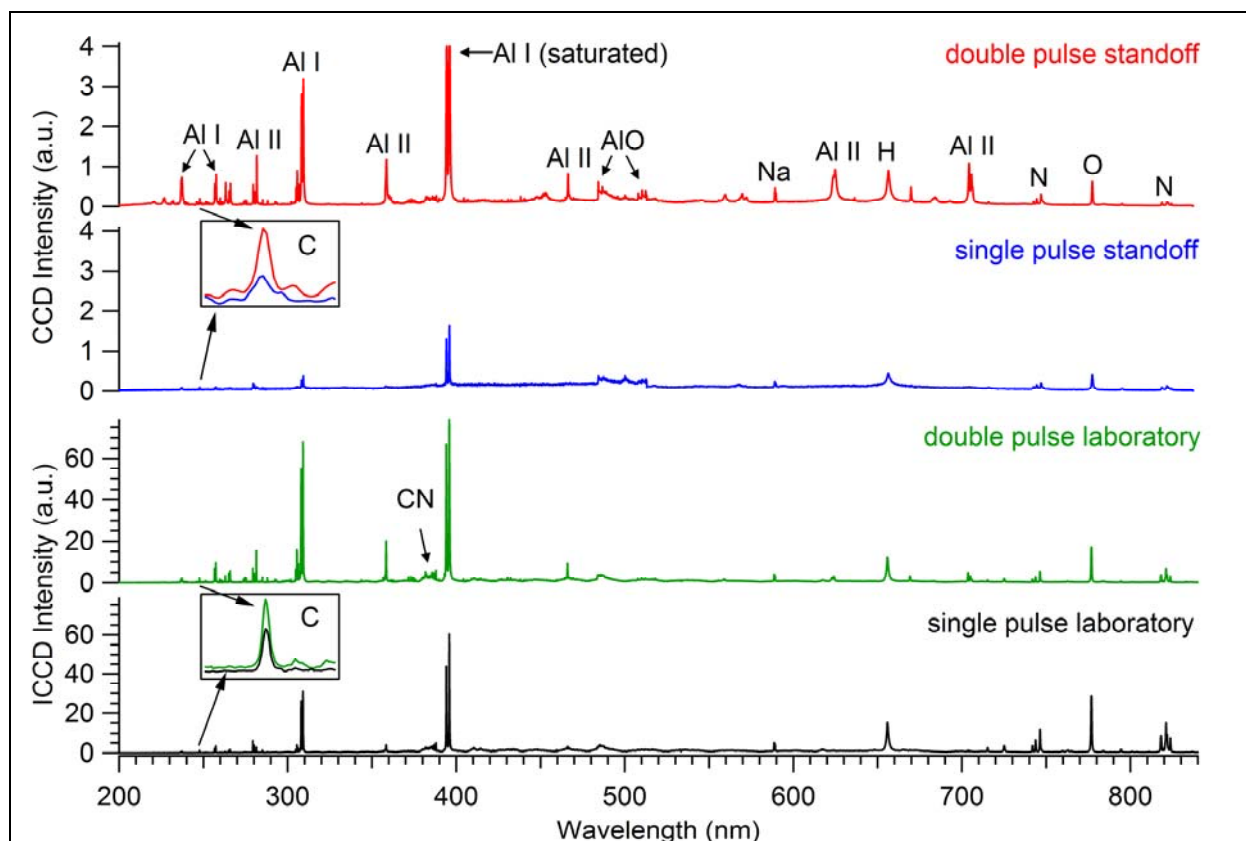
Figure 5. LIBS spectra (20 shots averaged) of RDX residue on Al (from top to bottom): at 20 m with a double pulse laser (275 mJ total energy, \Delta t=3\ \mu\text{s} , CCD spectrometer); at 20 m with a single 275 mJ pulse; at close contact with a double pulse laser (320 mJ total energy, \Delta t=2\ \mu\text{s} , ICCD spectrometer); and at close contact with a single 320-mJ pulse. (Strong emission lines are labeled for reference and the C line at 247 nm is inset and magnified on a 2-nm scale.)
