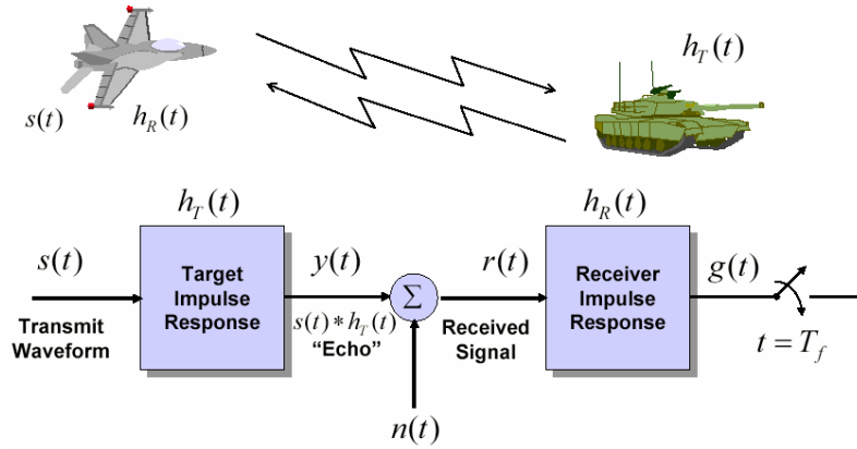
Figure 9: The Target-Matched Illumination Problem (after Guerçi [38]).
