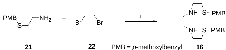
Scheme 3. Reagents: (i) CeOH, molecular sieve (4Å), DMF.
