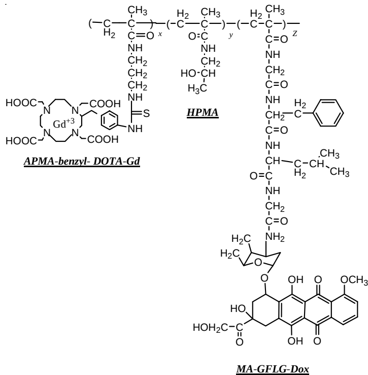
Figure 1. General structure of HPMA-copolymer-DOTA(Gd)-Dox conjugates.
