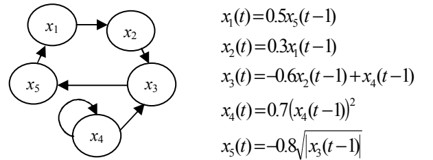
Figure 4. A simulated five-node network.
