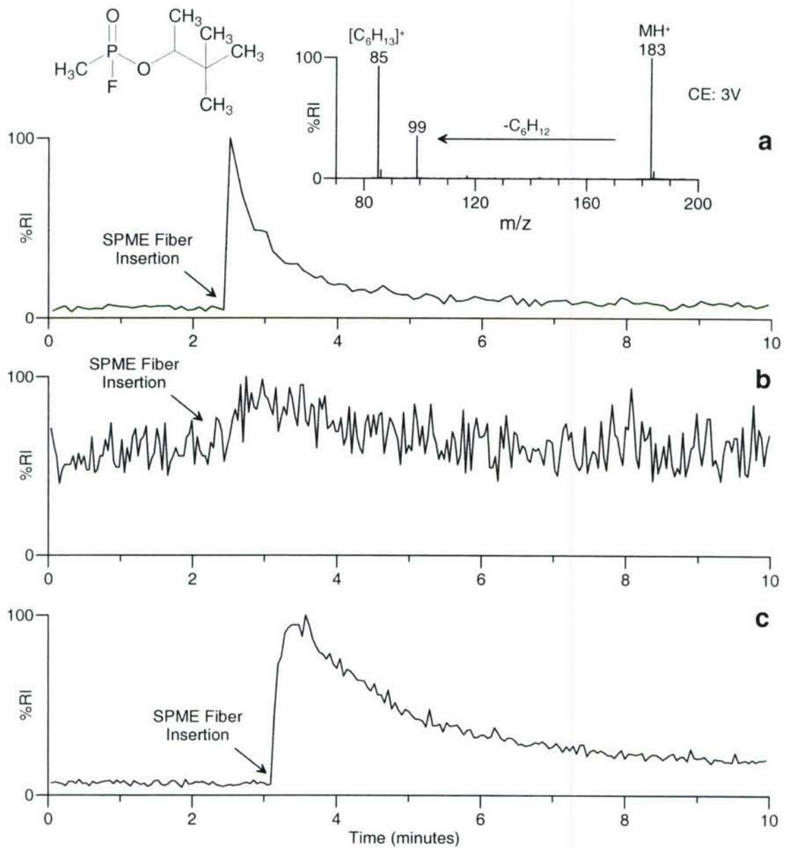
Figure 12. DESI-MS/MS chromatograms for m/z 183 obtained during analysis of a) a SPME fiber used to sample the headspace (15 s at 40 °C) above 5 \mu\text{g} of soman (GD), b) a SPME fiber used to sample the headspace (10 min at 40 °C) above canola oil spiked at the 10 \mu\text{g/g} level with GD and c) a SPME fiber used to sample the headspace (10 min at 40 °C) above corn meal spiked at the 10 \mu\text{g/g} level with GD. Inset: typical product ion mass spectrum for GD.
