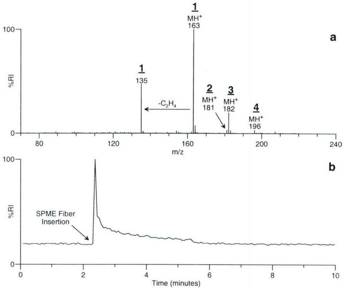
Figure 16. a) ESI-MS data acquired during DESI-MS analysis of a SPME fiber used to sample the headspace (10 min at 40 °C) above canola oil spiked at the 20 µg/g level with a munitions grade sample of tabun (GA). Tabun and three related compounds were detected. b) DESI-MS total-ion current (m/z 70 to 700) chromatogram obtained during this analysis.
