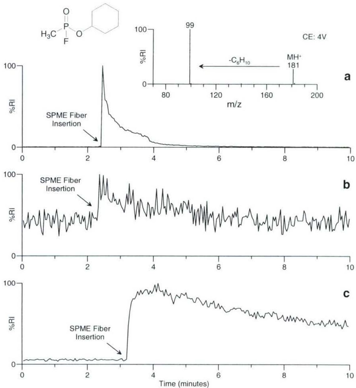
Figure 13. DESI-MS/MS chromatograms for m/z 181 obtained during analysis of a) a SPME fiber used to sample the headspace (15 sec at 40 °C) above 5 \mu\text{g} of cyclohexyl methylphosphonofluoridate (GF), b) a SPME fiber used to sample the headspace (10 min at 40 °C) above canola oil spiked at the 10 \mu\text{g/g} level with GF and c) a SPME fiber used to sample the headspace (10 min at 40 °C) above corn meal spiked at the 10 \mu\text{g/g} level with GF. Inset: typical product ion mass spectrum for GF.
