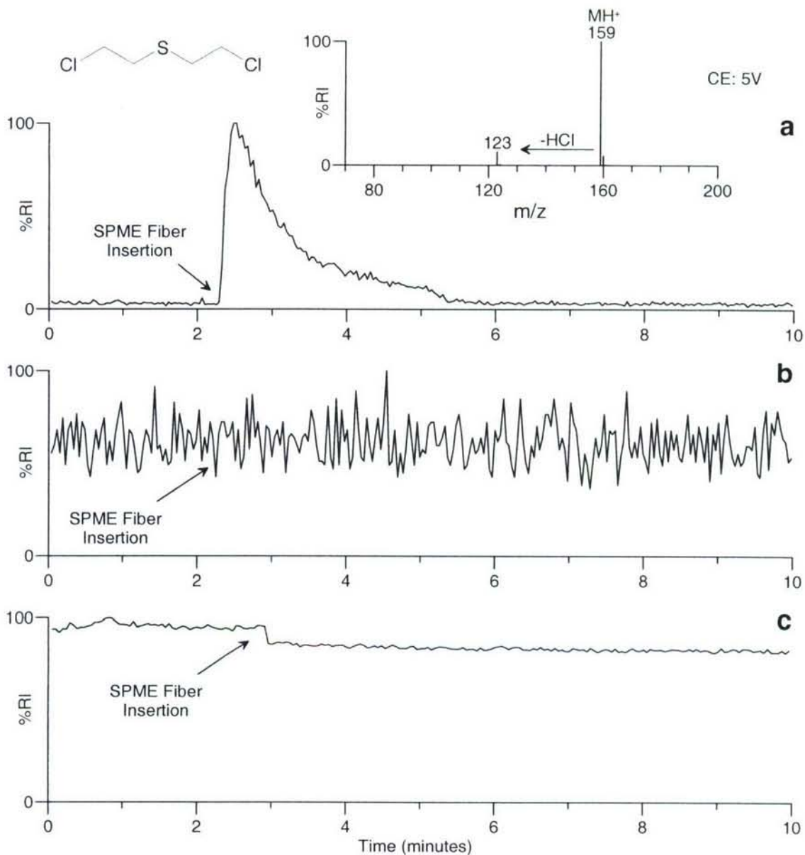
Figure 15. DESI-MS/MS chromatograms for m/z 159 obtained during analysis of a) a SPME fiber used to sample the headspace (10 min at 40^{\circ}\text{C} ) above 10\ \mu\text{g} of mustard (H), b) a SPME fiber used to sample the headspace (10 min at 40^{\circ}\text{C} ) above canola oil spiked at the 10\ \mu\text{g/g} level with H and c) a SPME fiber used to sample the headspace (10 min at 40^{\circ}\text{C} ) above corn meal spiked at the 10\ \mu\text{g/g} level with H. Inset: typical product ion mass spectrum for H.
