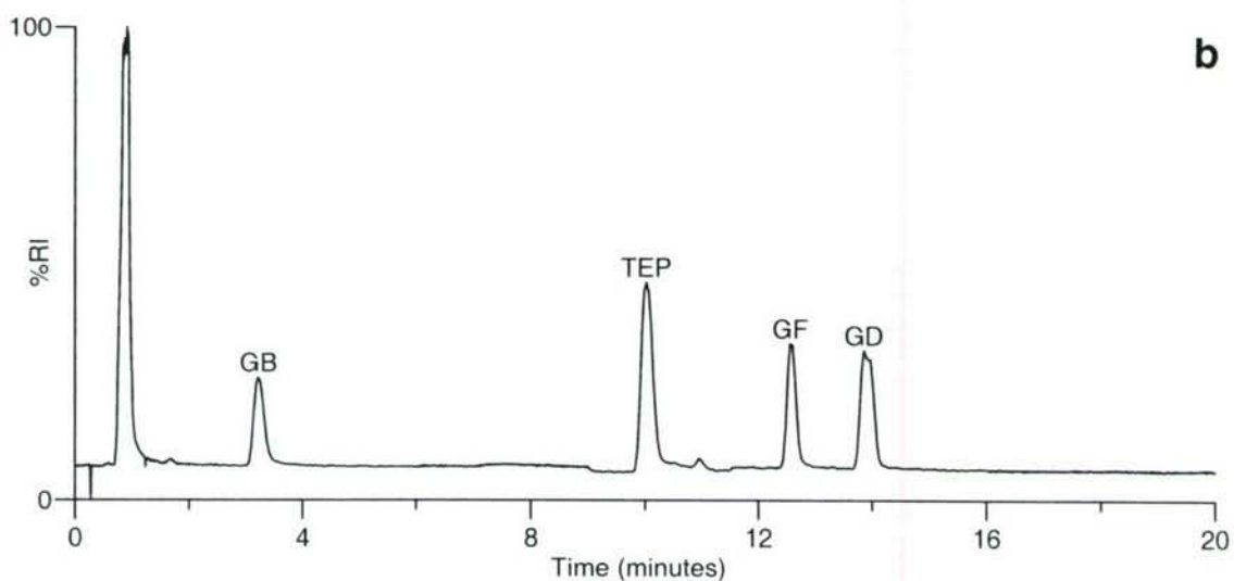
Figure 1. LC-ESI-MS total-ion-current ( m/z 70 to 500) chromatogram for a) bottled water blank and b) bottle water spiked at the 10 \mu\text{g/mL} level with sarin (GB), triethyl phosphate (TEP), cyclohexyl methylphosphonofluoridate (GF) and soman (GD). Product ion mass spectra for the [M+H]^+ ion for each of the spiked compounds were also acquired during this analysis. Product mass spectra for m/z 141, m/z 183, m/z 181 and m/z 183 were acquired from 2 to 6 min, 9 to 11.5 min, 11.5 to 13.3 min and 13.3 to 16 min, respectively (refer to Figure 2).
