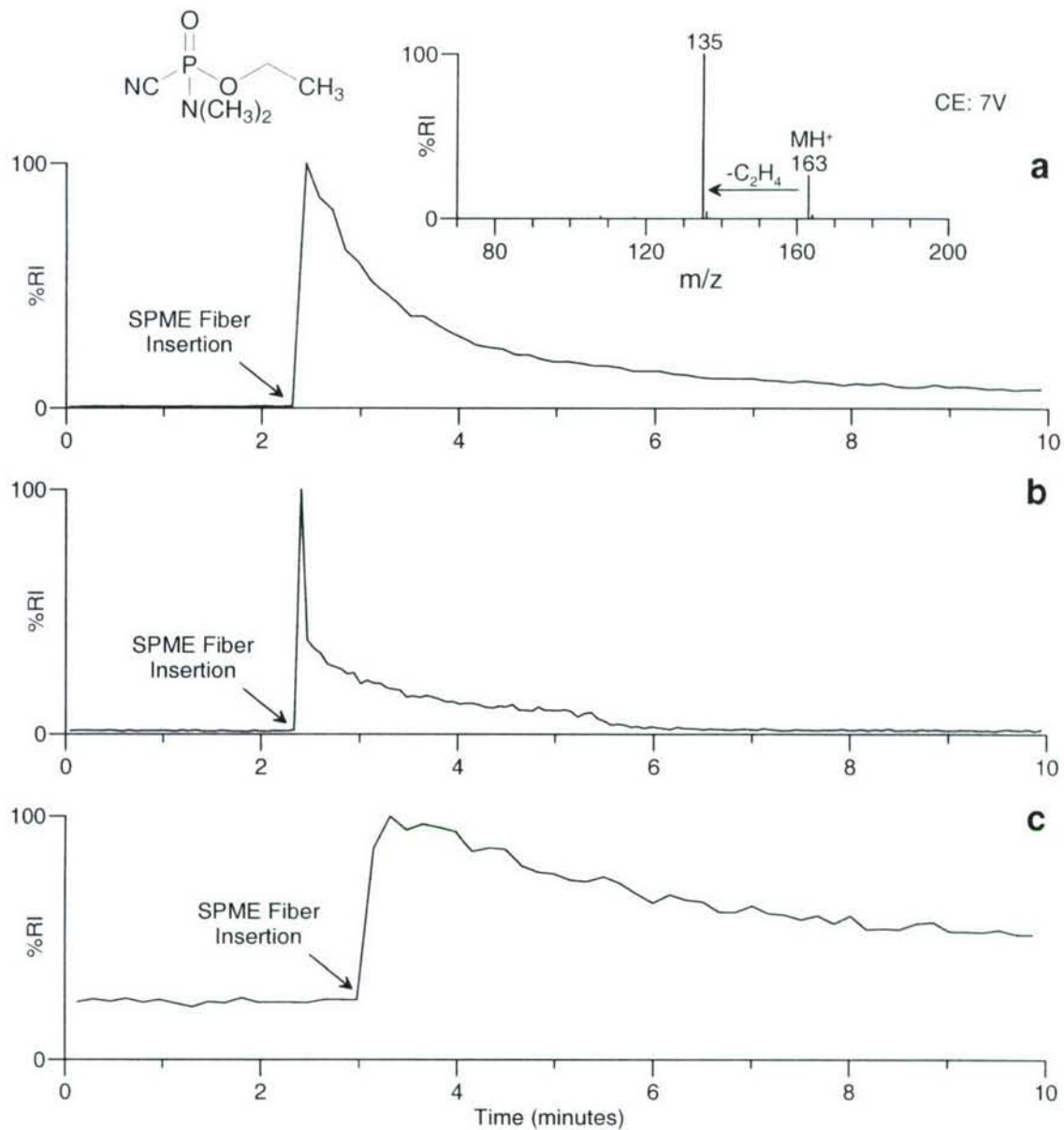
Figure 11. DESI-MS/MS chromatograms for m/z 163 obtained during analysis of a) a SPME fiber used to sample the headspace (2 min at 40 °C) above 0.5 \mu\text{g} of tabun (GA), b) a SPME fiber used to sample the headspace (10 min at 40 °C) above canola oil spiked at the 15 \mu\text{g/g} level with GA and c) a SPME fiber used to sample the headspace (10 min at 40 °C) above corn meal spiked at the 15 \mu\text{g/g} level with GA. Inset: typical product ion mass spectrum for GA.
