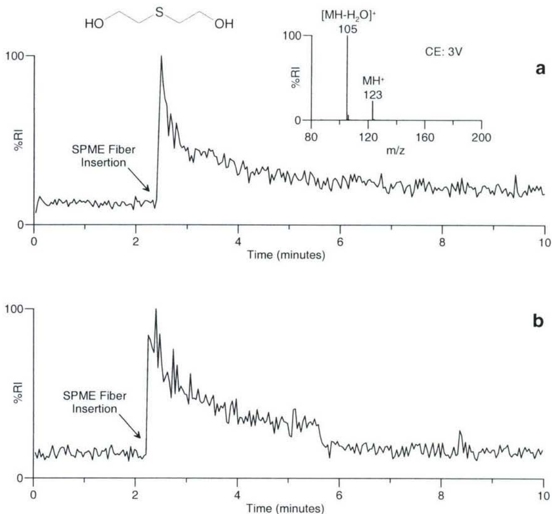
Figure 20. DESI-MS/MS chromatograms for m/z 123 obtained during analysis of a) a SPME fiber used to sample the headspace (10 min at 80 °C) above 5 \mu\text{g} of thiodiglycol and b) a SPME fiber used to sample the headspace (10 min at 80 °C) above canola oil spiked at the 20 \mu\text{g/g} level with thiodiglycol. Inset: typical product ion mass spectrum for thiodiglycol.
