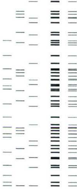
Figure 15: Superimposed temporal sequences
