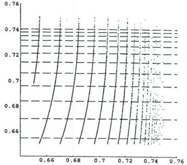
Figure 6: Mapping T_{n_{k+1}} = h(T_{n_k}) . Final intervals T_{n_{k+1}} are shown vertically versus preceding final intervals T_{n_k} (horizontally). Counting from the left, d_{k+1} is the number of the graph branch. Dashed lines separate variable ranges occupied by the branches.
