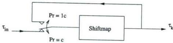
Fig. 6. Frobenius filter is a shift map with input. Either the input interval \tau_{in} or the present output interval \tau_k is transformed into the next output interval \tau_{k+1} .
