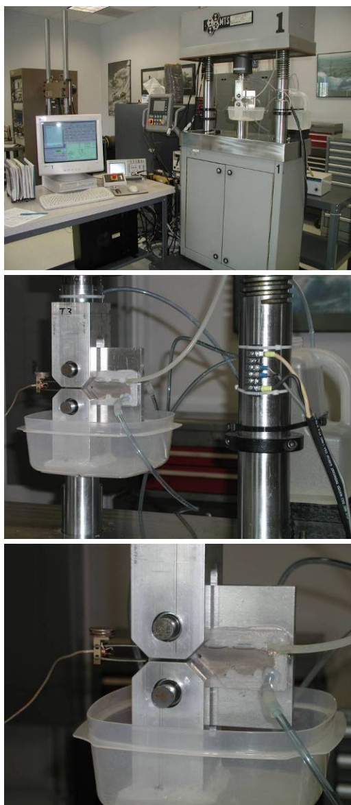
Figure 2. Photographs of test equipment and test set-up (seawater environment).
