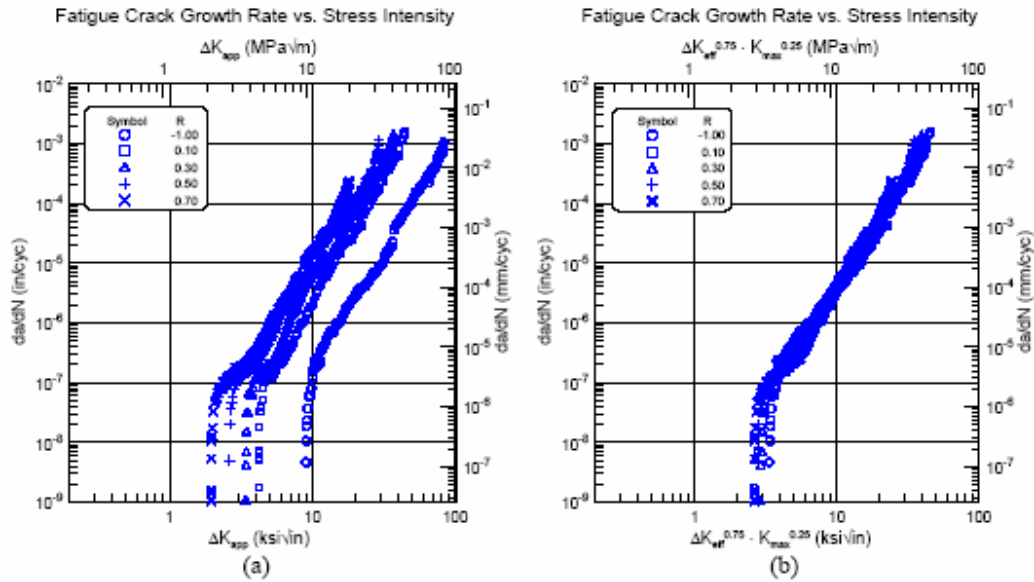
Fig. 5. Fatigue crack growth data of 2324-T39 Al showing: (a) \Delta K_{app} and (b) K_{norm} after ACR correction.
