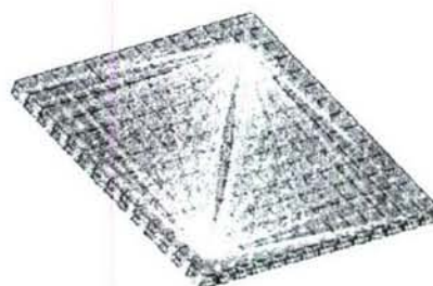
Figure 3 3-D mesh of square PWAS with boundary conditions
