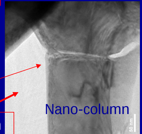
TEM image of a re-growth junction
