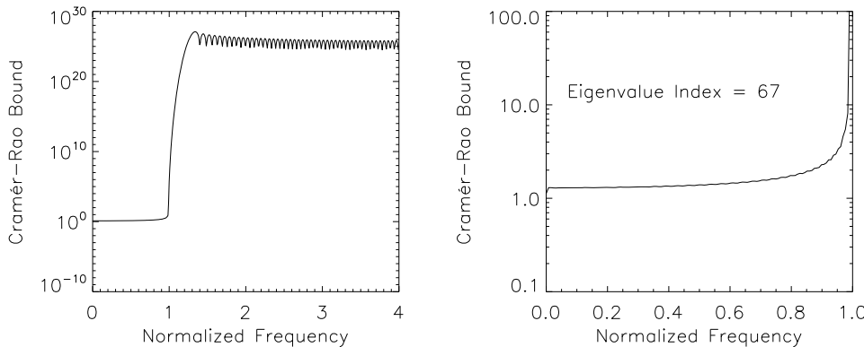
Fig. 5. A movie of the CRBs for any unbiased estimate of any Fourier spectra for a SBP of 40 plotted as a function of frequency normalized to one at the edge of the measurement bandwidth. Each movie frame corresponds to adding one additional eigenvalue to the pseudoinverse of the FIM. The plots on the left are for all frequencies included in the calculations, while the plots on the right are a magnified version of the plots on the left for frequencies within the
