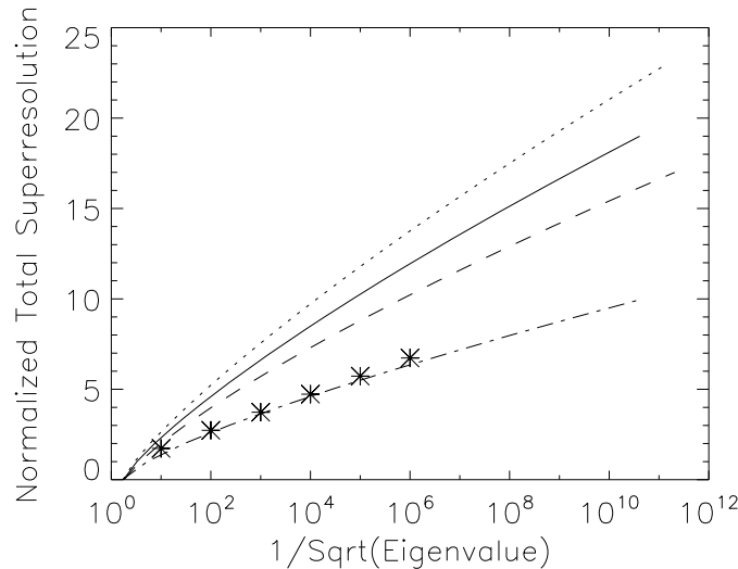
Fig. 9. Plots of the increases in the PSWF-defined degrees of freedom averaged over the entire support region brought about by including both primary and secondary superresolution in the reconstruction process. The dot-dash line is for a SBP of 1.27, the dashed line is for a SBP of 10, the solid line is for a SBP of 20, and the dotted line is for a SBP of 40. The asterisks denote values calculated in [1] for a SBP of 1.27.
