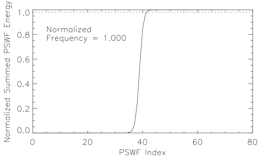
Fig. 6. A movie of the total energy of the PSWFs included in the reconstruction process (normalized to one) as a function of the PSWF index for a SBP of 40. The dotted line corresponds to a value of 0.98. Each frame of the movie corresponds to a different superresolved frequency as indicated in the movie.
