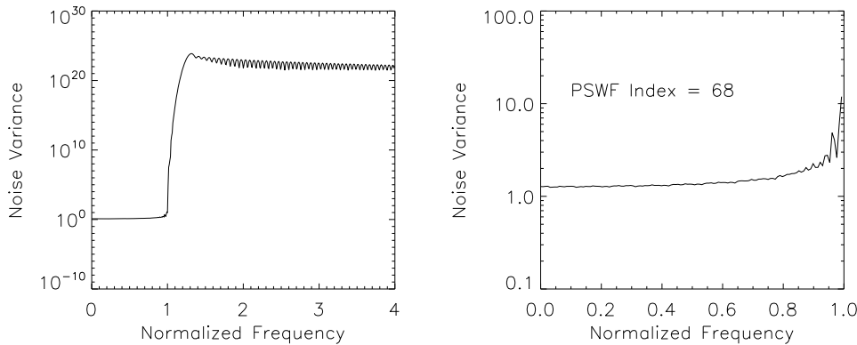
Fig. 3. A movie of the Fourier variances defined by Eq.(3) for a SBP of 40 plotted as a function of frequency normalized to one at the edge of the measurement bandwidth. Each movie frame corresponds to increasing the finite summation limit in Eq.(3) by one. The plots on the left are for all frequencies included in the calculations, while the plots on the right are a magnified version of the plots on the left for frequencies within the measurement bandwidth.
