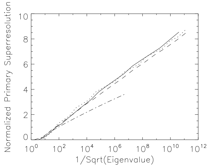
Fig. 7. Plots of the increases in the sampling degrees of freedom in superresolved reconstructions brought about by including primary superresolution spectra. The dot-dash line is for a SBP of 1.27, the dashed line is for a SBP of 10, the solid line is for a SBP of 20, and the dotted line is for a SBP of 40.
