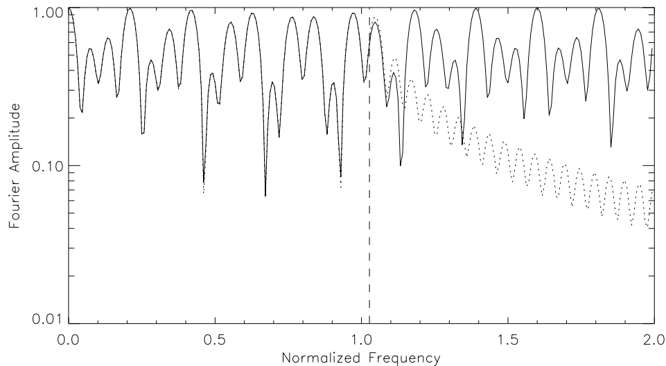
Fig. 8. Plots of the Fourier amplitudes of a triple star for the parameters listed in the text. The solid line is a plot of the true Fourier amplitudes and the dotted line corresponds to a reconstruction of the true Fourier amplitudes using Eq.(2) with an upper limit of 46 and a SBP of 40. The frequency axis is normalized to one at the edge of the measurement bandwidth, and the dashed line indicates the upper boundary of the primary superresolution region.
