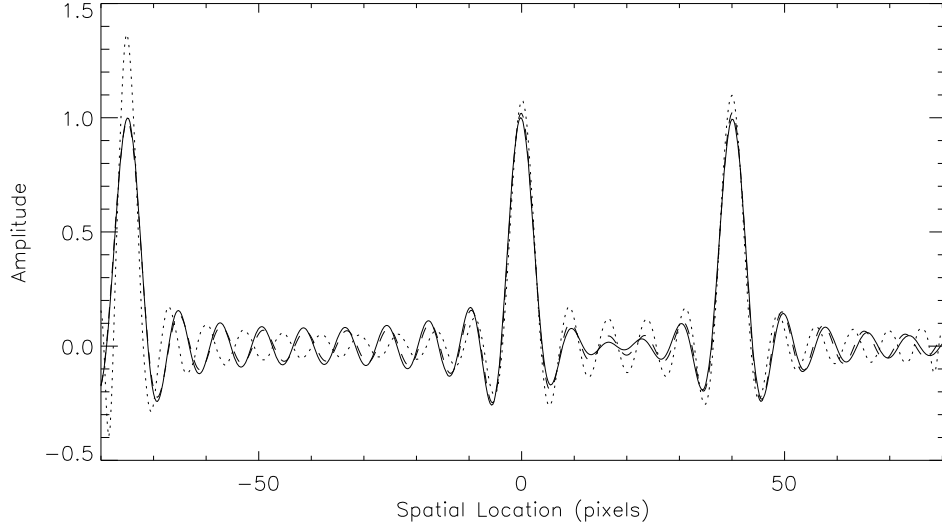
Fig. 13. Plots of reconstructions of the triple star whose Fourier amplitudes are shown in Fig. 8, where the solid line is a reconstruction using just the Fourier data inside the measurement bandwidth, the dashed line is a reconstruction using both the measured Fourier data and the primary superresolution part of the superresolved spectrum, and the dotted line is a reconstruction using the measured Fourier data and all of the superresolved spectrum.
