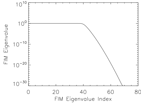
Fig. 4. A plot of the FIM eigenvalues.
