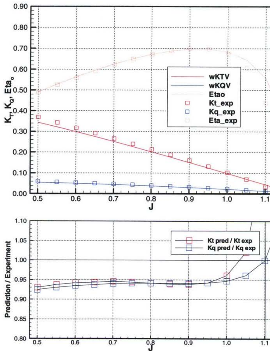
Figure B- 4. Propeller 5426 open water prediction.
