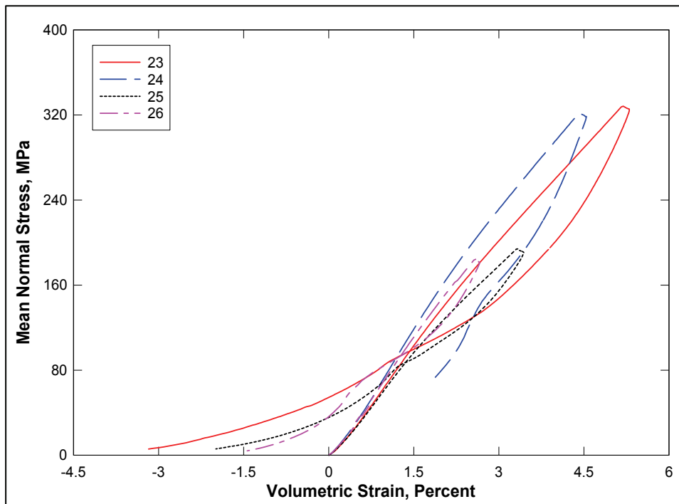
Figure 36. Pressure-volume data from UX/BX tests
