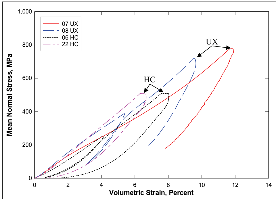
Figure 34. Comparison of pressure-volume data from HC and UX tests
