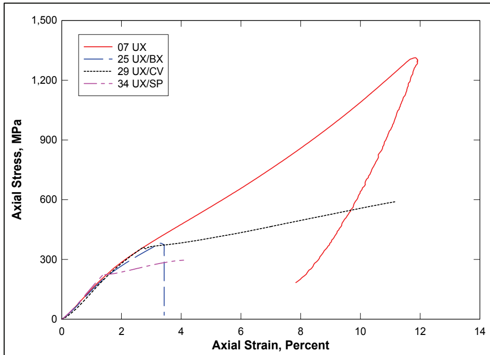
Figure 47. Stress-strain curves from selected UX, UX/BX, UX/CV, and UX/SP tests
