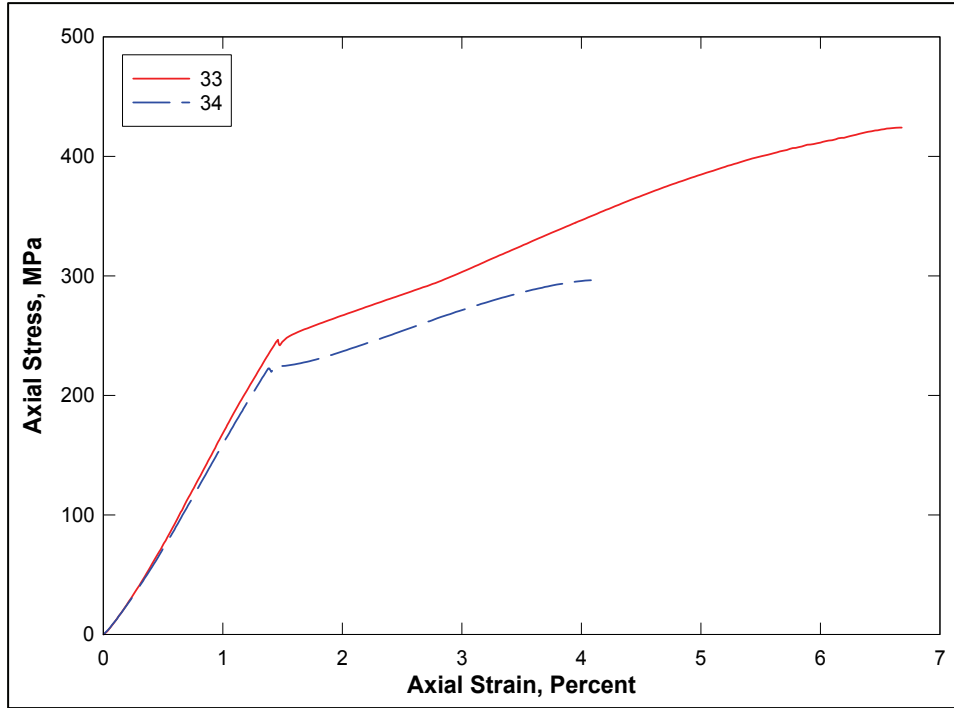
Figure 43. Stress-strain curves from UX/SP tests
