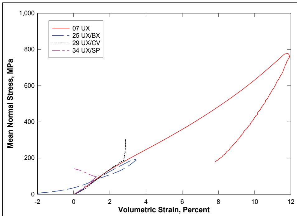
Figure 48. Pressure-volume data from selected UX, UX/BX, UX/CV, and UX/SP tests
