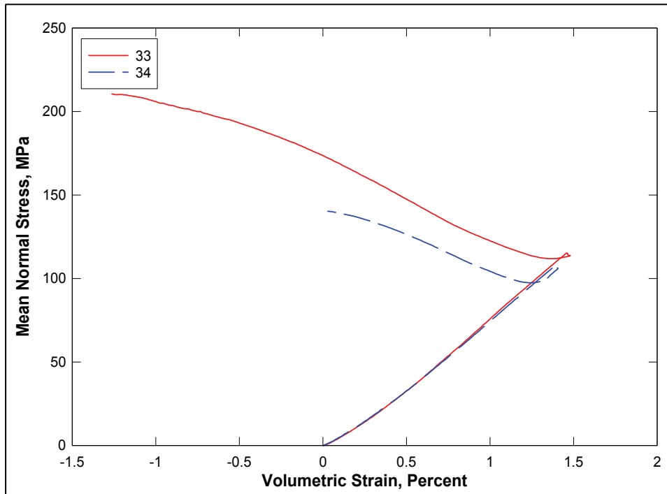
Figure 44. Pressure-volume data from UX/SP tests
