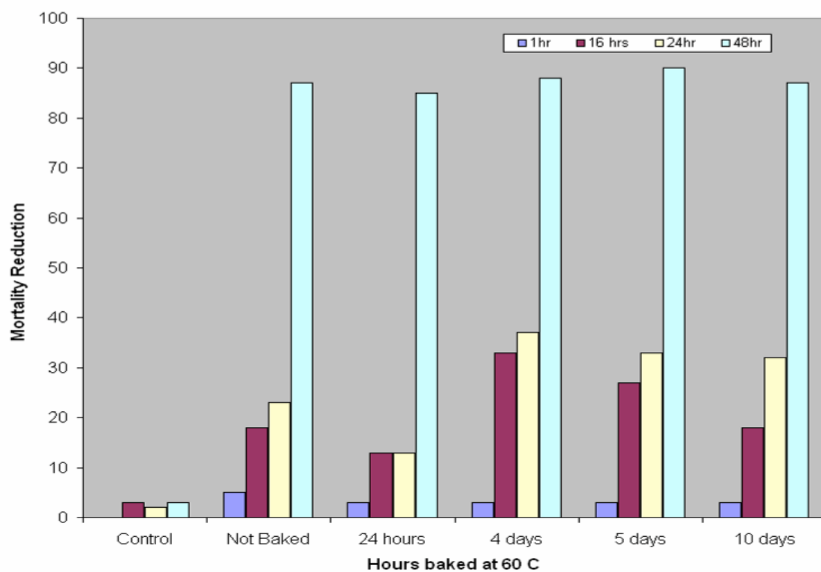
Figure 15. Percent mortality of house flies exposed to MaxForce spot fly bait applied to wood blocks and oven-aged at 60°C for 1, 4, 5, and 10 days.
