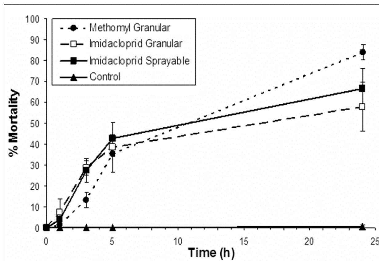
Figure 10. Mortality of female house flies exposed to imidacloprid and methomyl granular scatter baits and a sprayable imidacloprid bait.
