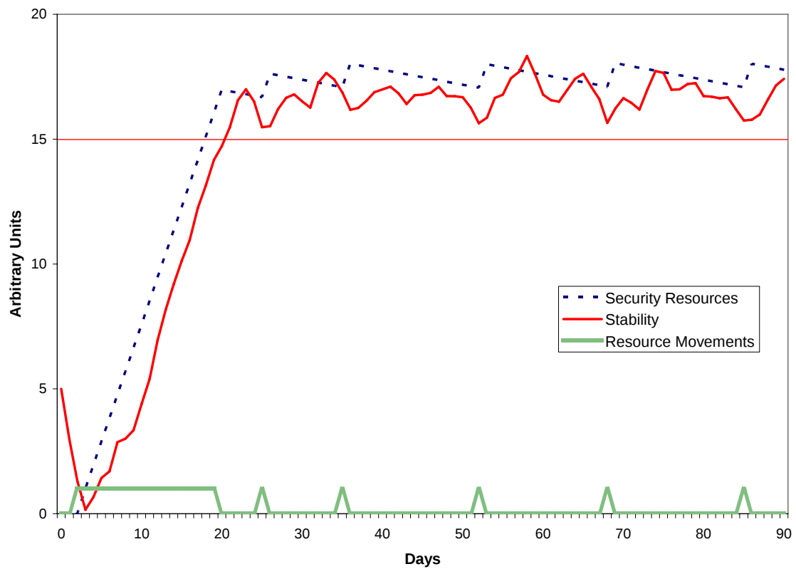
Figure 2: Benchmark run for model A1. The red horizontal line indicates the stability threshold.
