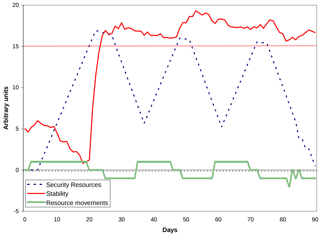
Figure 3: Benchmark run for model A2. The red horizontal line indicates the stability threshold.
