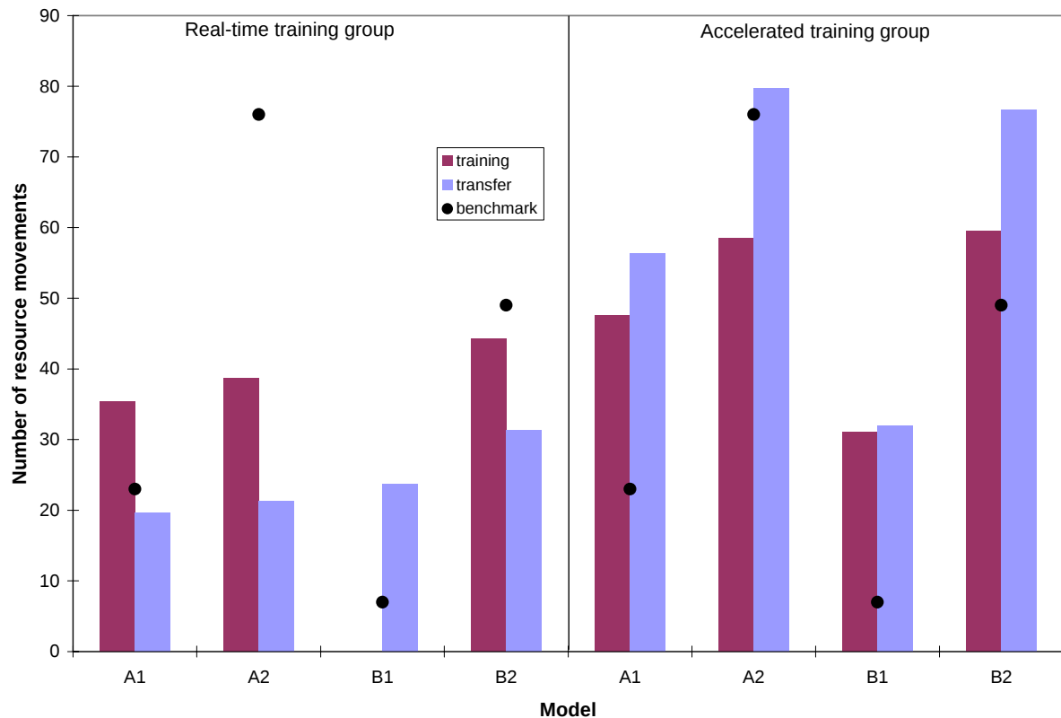
Figure 10: Number of resource movements by model for each training group. Training data for model B1 for the RT group and for one of the participants in the accelerated group are unavailable
