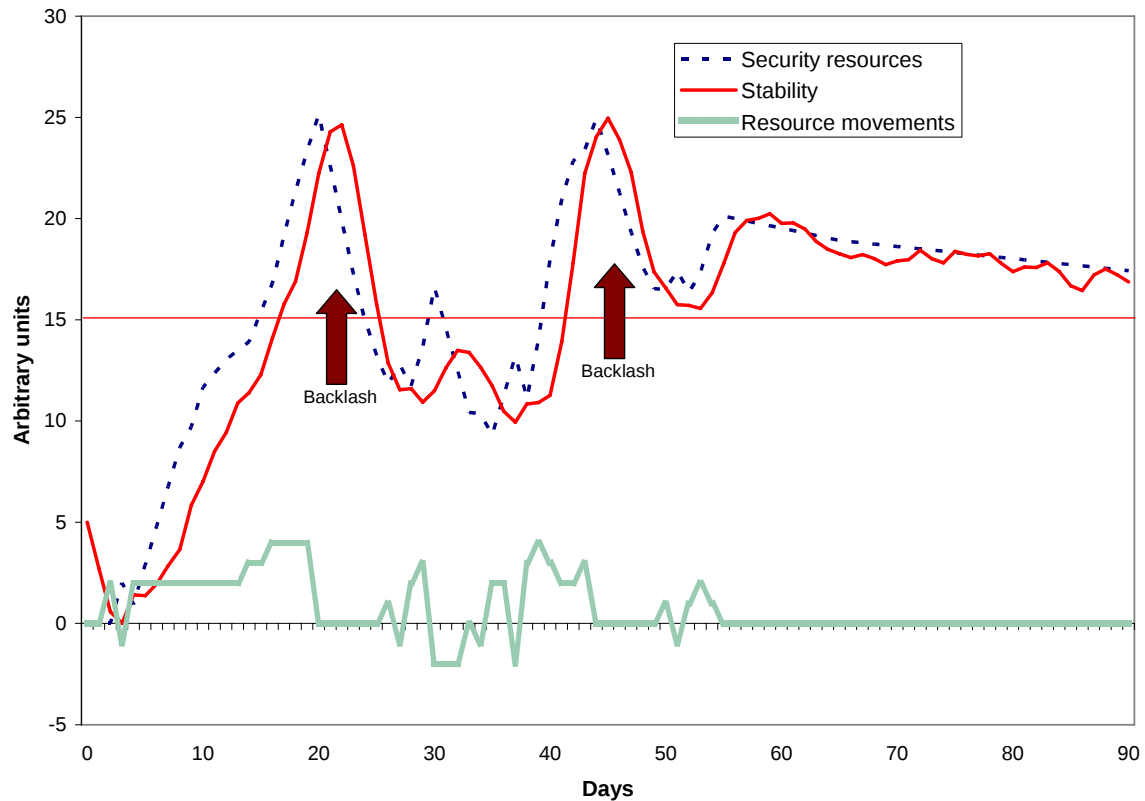
Figure 13: Sample run from the transfer session by one participant(accelerated training group) showing oscillations in the stability index due to backlash from excessive resource movements (i.e., a drop in resource levels without a corresponding withdrawal of resources by the participant) for model A1, a “stabilize-and-stay” model requiring slow resource build-up. The horizontal red line at 15 units marks the desired stability level.
