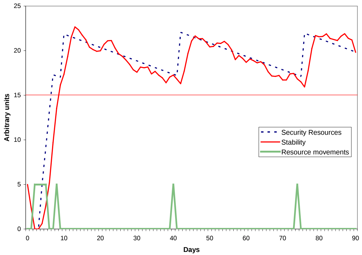
Figure 4: Benchmark run for model B1
