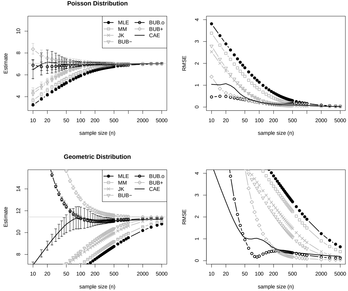
Figure 4: The two distributions considered here have infinite support, with m = \infty . (Left) The estimated entropy for several different estimators, over a range of sample sizes n . The lines are average estimates taken over 1,000 independent realizations, and the vertical bars indicate \pm one standard deviation of the estimate. The actual value of H is indicated by a solid gray horizontal line. MM and JK are the Miller-Maddow and Jackknife corrected MLEs. BUB-, BUB.o, and BUB+ are the BUB estimator with its m parameter set to a naive \hat{m} , oracle m = \lceil 2^H \rceil , and twice the oracle m . CAE is the coverage adjusted estimator. (Right) The corresponding root mean squared error (RMSE). Results are very similar to those in the previous figure, the CAE estimator performs nearly as well as the oracle BUB.o.
