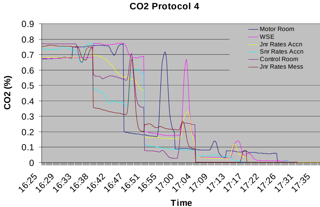
Figure 3. The CO 2 concentration in the living and working areas of the submarine during a one hour and 10 minute snort.
