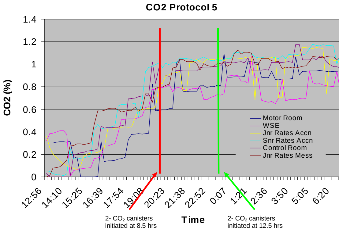
Figure 4. Changes in CO 2 concentration and the effects of air purification scrubbing under sonar quiet conditions. Two CO 2 canisters were activated simultaneously in both the Fore Ends (foreword of Bulkhead 34 upper deck WSC) and the After Ends (Motor Room aft of Bulkhead 56) at 2010 and 2410, respectively.
