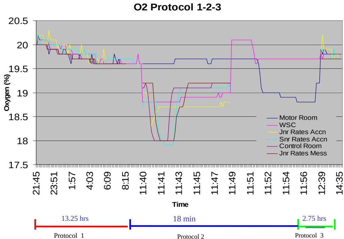
Figure 2. Changes in O 2 concentrations under patrol and snort conditions within six working and living areas of the submarine.
