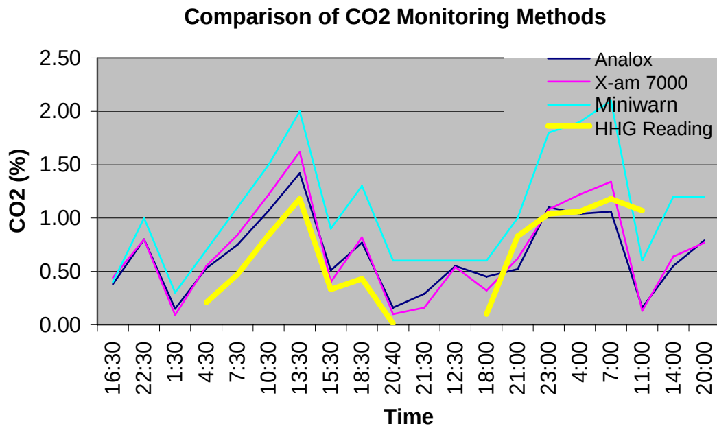
Figure 8. Comparison of CO 2 readings between study detection equipment and potential replacement monitors during the three day habitability trial (data includes CO 2 readings during all five protocols, monitoring dived and snort protocols. Replacement monitors also monitored during non-study periods as part of standard operating procedures).
