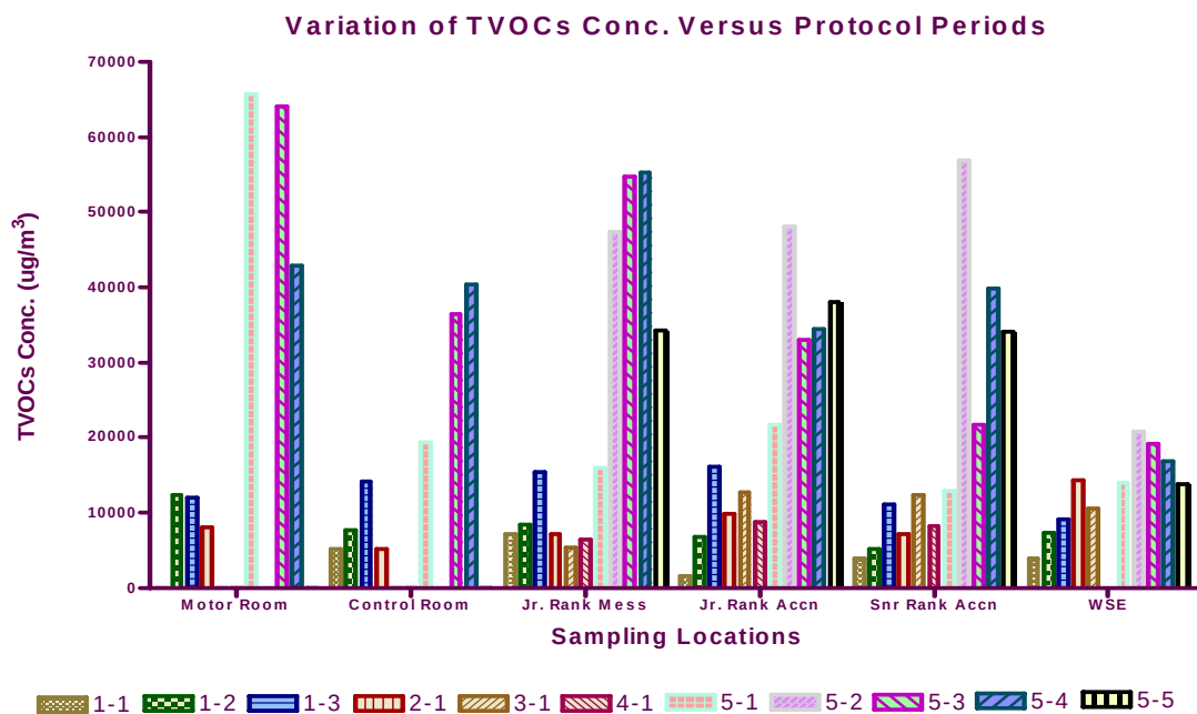
Figure 7. Total Volatile Organic Compound (TVOCs) concentration variation for each collection period in each protocol within the six compartments of the submarine (TVOCs includes over 300 compounds consisting of aromatics, aliphatics and fluorocarbons).
