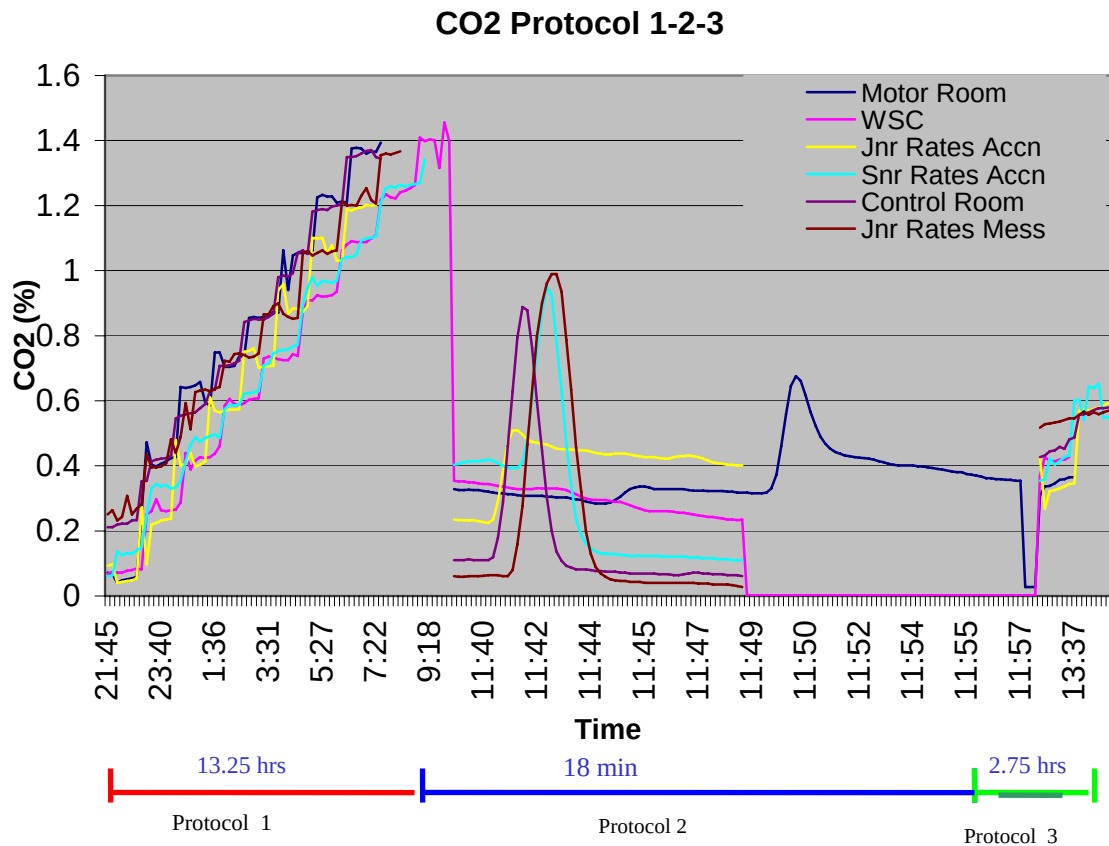
Figure 1. Changes in CO 2 concentrations under patrol state and snort conditions within six working and living areas of the submarine.
