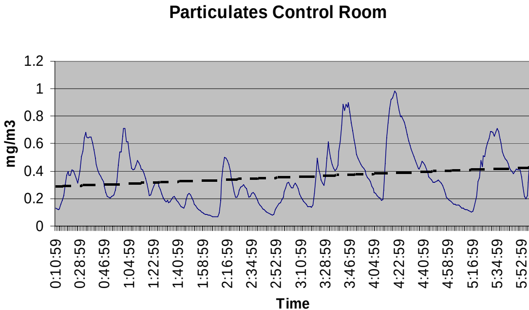
Figure 6. The total inhalable particulates ( > 10\ \mu\text{m} ) continuously measured in the control room over an 8 hour period.
