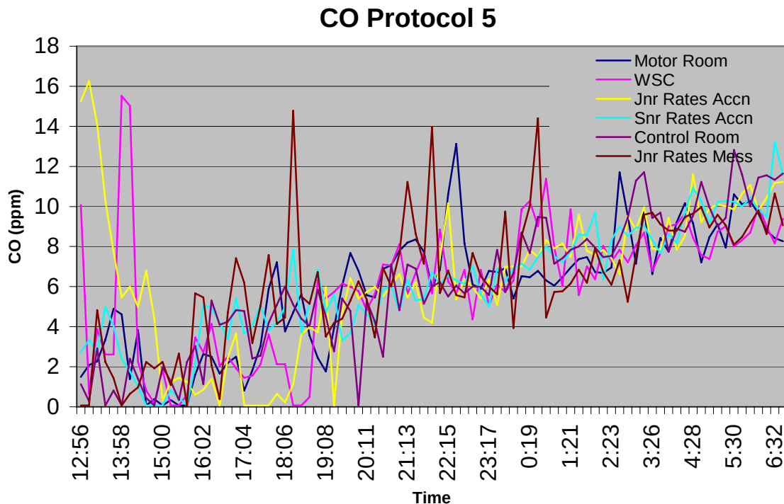
Figure 5. Changes in CO concentrations during sonar quiet condition (one motor running, one fan on slow).
