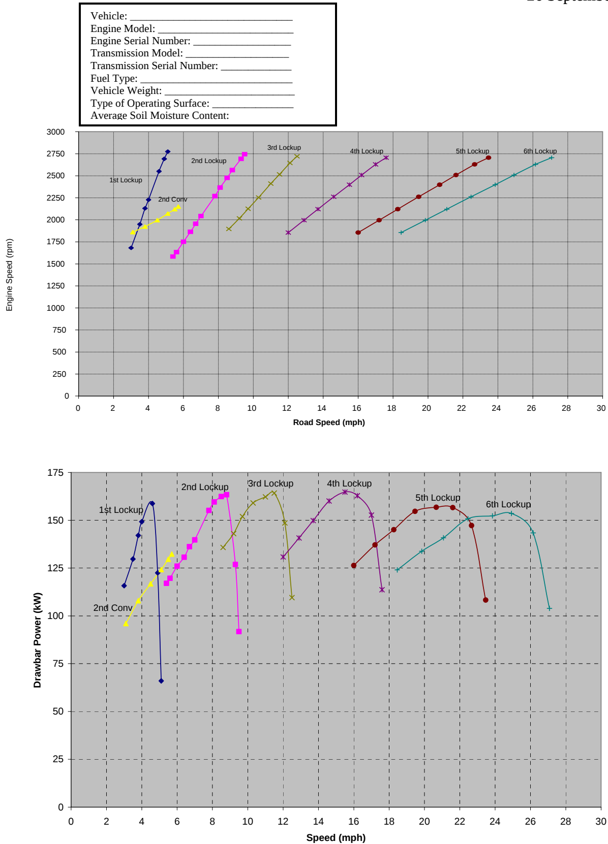
FIGURE 2. Drawbar power characteristics
