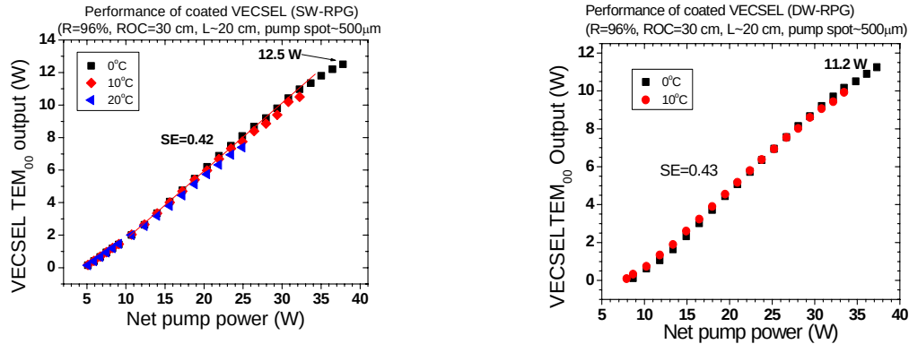
FIGURE 3. VECSEL \text{TEM}_{00} output vs. net pump power: SW-RPG VECSEL (left) and DW-RPG VECSEL (right).
