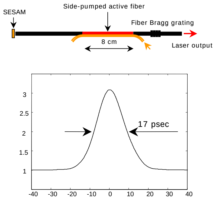
Figure 24. Top: Schematic diagram of the short fiber-laser oscillator modelocked with a semiconductor saturable-absorber mirror (SESAM). The fundamental pulse repetition rate of the oscillator is 550MHz. Bottom: Autocorrelation trace of the transform-limited pulse generated by the source.
