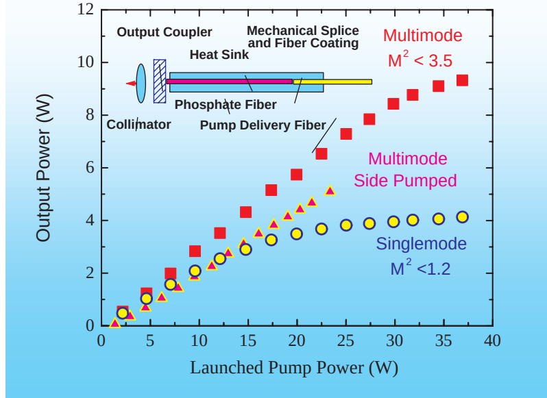
Fig 2. Performance of 7 cm multimode (squares) and single mode (circles) end-pumped fiber lasers, and 12 cm side-pumped multimode fiber laser (triangles). The inset shows the schematic layout of the end-pumped fiber laser.
