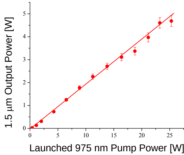
Fig. 5. Signal vs. launched pump power of a 3.5-cm phosphate microstructured fiber laser.
