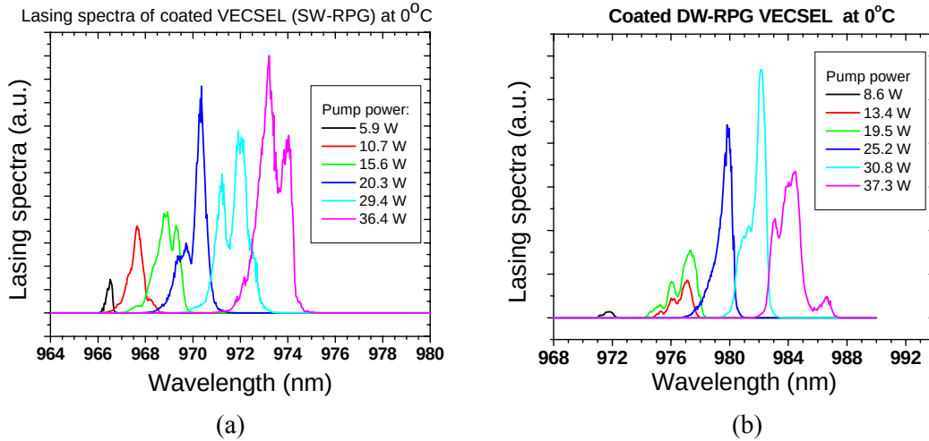
FIGURE 5. Lasing spectra of VECSEL at different pump power: (a) SW-RPG VECSEL and (b) DW-RPG VECSEL.
