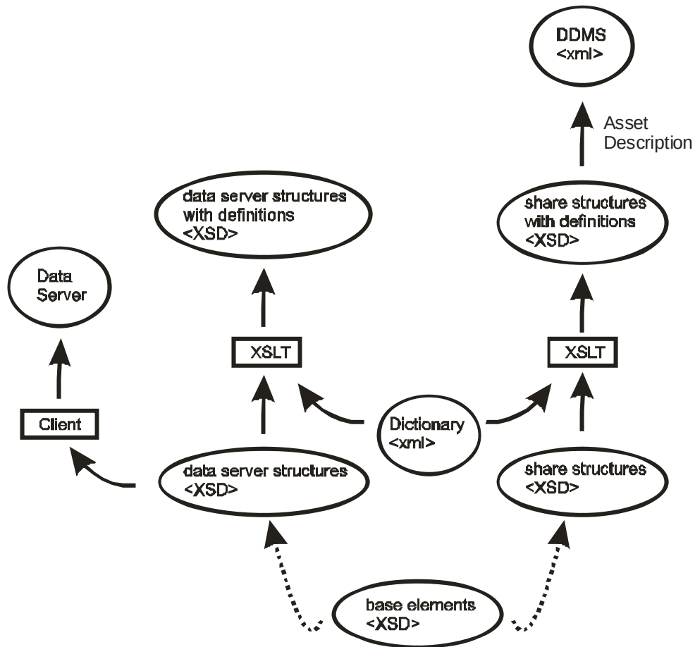
Figure 5: An architecture that takes advantage of the XML dictionary of terms and programmer created schemas. Programmers would create a set of base elements, including those elements in both the structures for private (data server structures) and public access (share structures). XSLT would be used to document the share structures using a consistent set of descriptions in the dictionary.
