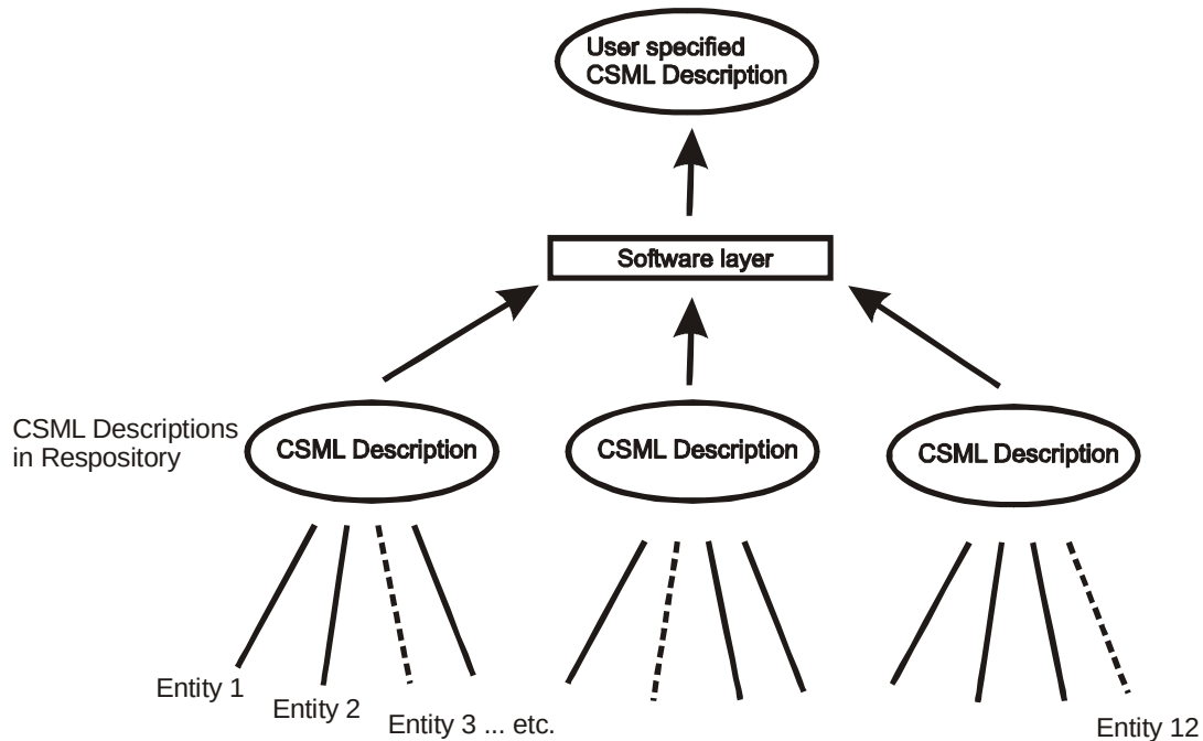
Figure 2: Conceptual model of how CSML metadata combine multiple data entities into a single data set as specified by the user. The dashed line indicates the entities identified as meeting user needs. These entities are from disparate data sources. The entity metadata records are combined to form a single, consistent CSML description for the user.
