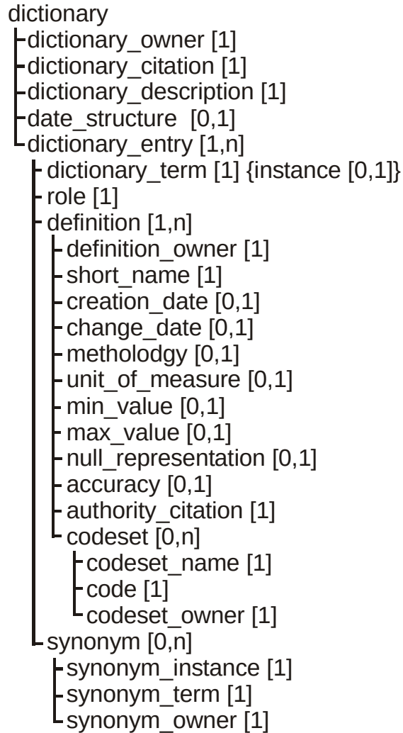
Figure 4: Schematic of the SGXML dictionary structure being proposed for the NUW project.
