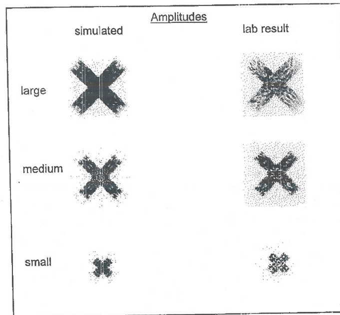
Figure 7. Each preselected amplitude shape was employed in three different sizes. The large size was approximately as broad as the diameter of the input beam.
