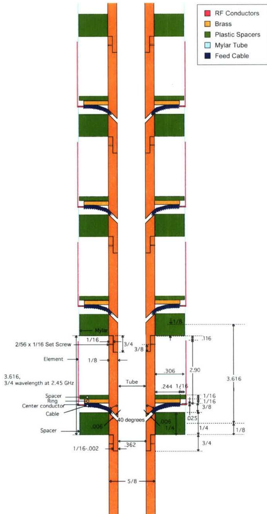
Figure 4-4. Four-Element QHA Array Assembly
