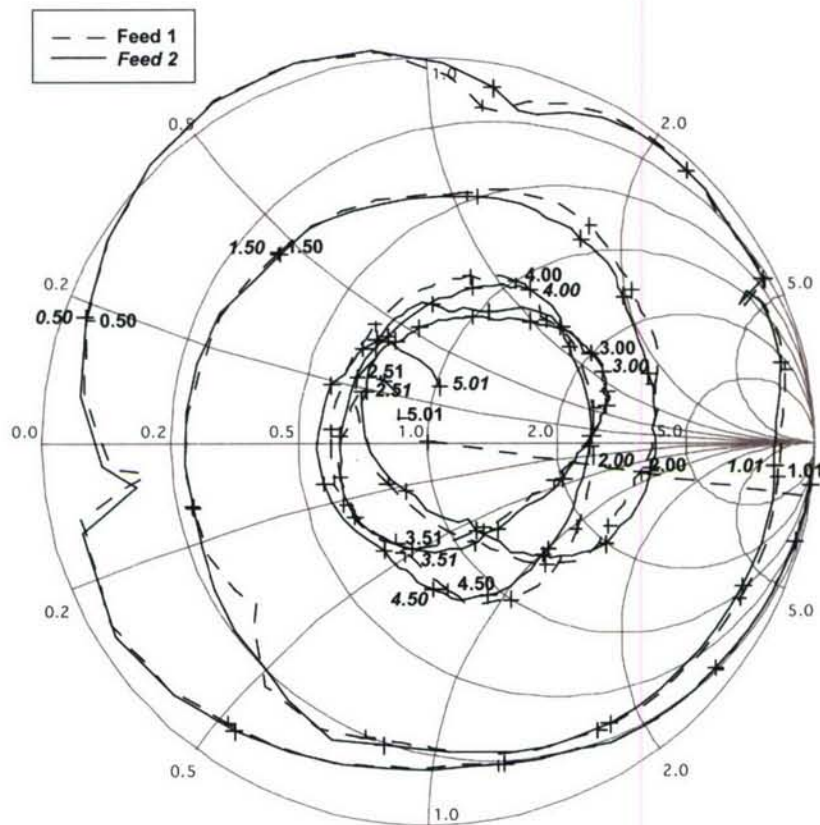
Figure 5-5. Smith Chart of the Measured Input Impedance of Both Bifilar Feeds of the Final QHA Element Design (Pitch Angle = 30°, Diameter = 1.224 in., Axial Length = 2.90 in. with an Enclosed Section of Brass Tube
