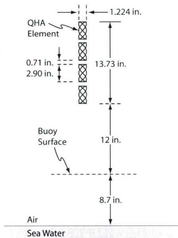
Figure 4-1. Four-Element Linear Array of QHA Elements Describing (a) Installation on a Buoy and (b) Array Geometry with Dimensions of Array Elements and Their Locations Relative to Buoy Surface and Air-Sea Water Interface
