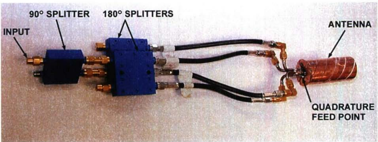
Figure 3-6. Constructed QHA: (a) Closeup View of Antenna and (b) Antenna Connected to Feed Network
