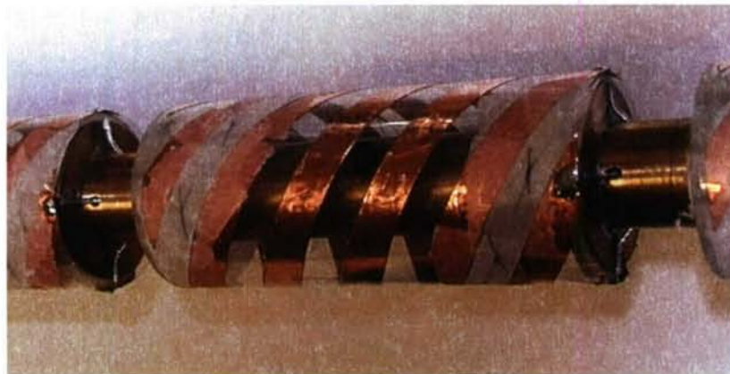
Figure 4-9. Closeup View of QHA Element Showing Feeds and Spacers
