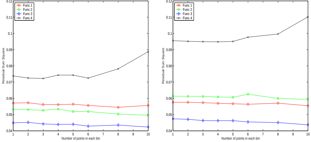
Figure 2: Mean square errors of the binned estimators v.s the number of data points in each bin. Left: Binned Periodic Gaussian kernel regularization; Right: Binned Gaussian kernel regularization. In both plots, unbinned estimators are those with 1 data in each bin.
