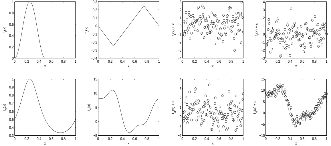
Figure 1: Regression functions and data used in the simulations.
