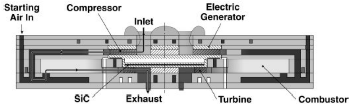
Figure 12 - MIT Designed MEMS Turbogenerator [41]
