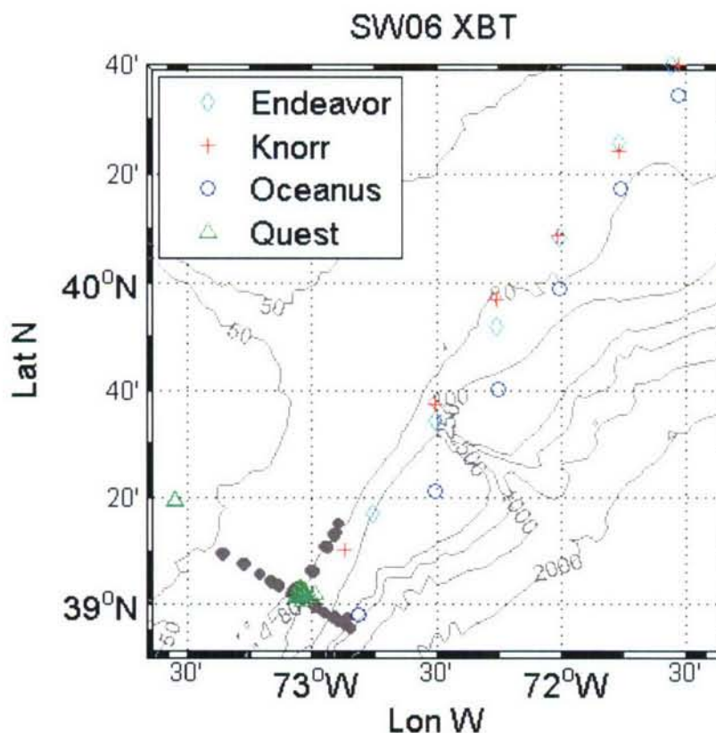
Figure 10.2 XBT stations performed during SW06.
