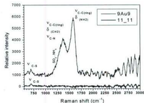
Fig. 5. Raman spectra of 35 nm LbL film (black) and after
