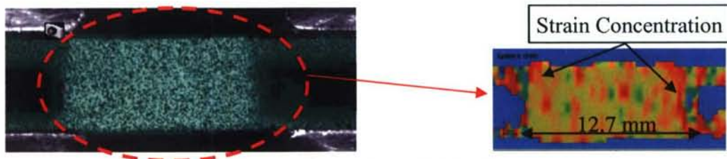
Figure 2.29: Strain Concentration in a D6641 Specimen
